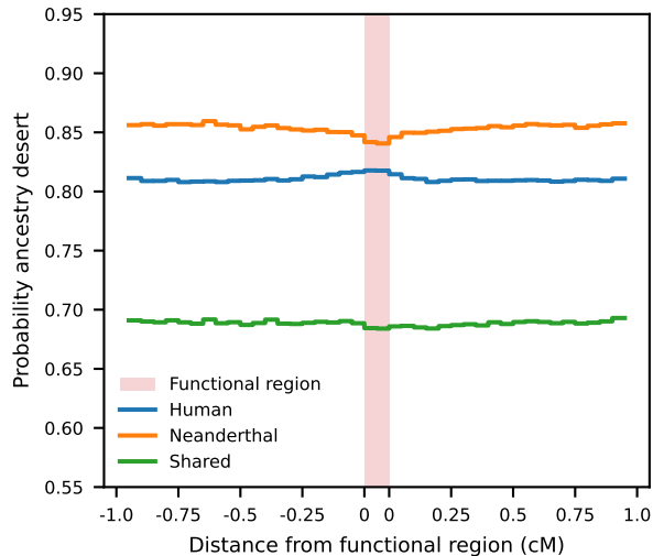
Directional selection, with mean = -0.0002 , shape = 0.5 , and \mu = 0.01
