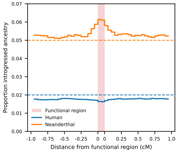
Directional selection, with mean = -0.001 , shape = 0.5 , and \mu = 0.01
