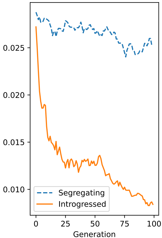
Neanderthal branch
