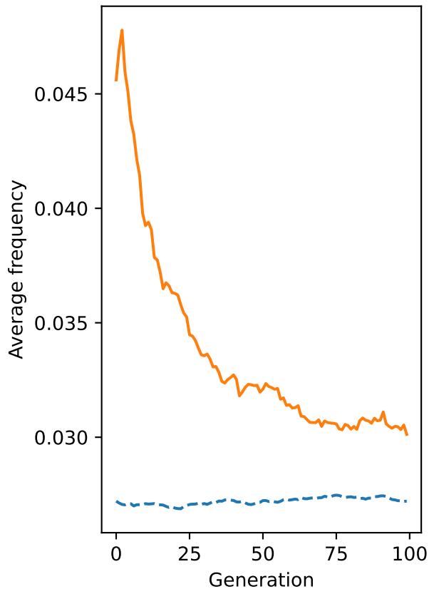
Human branch
