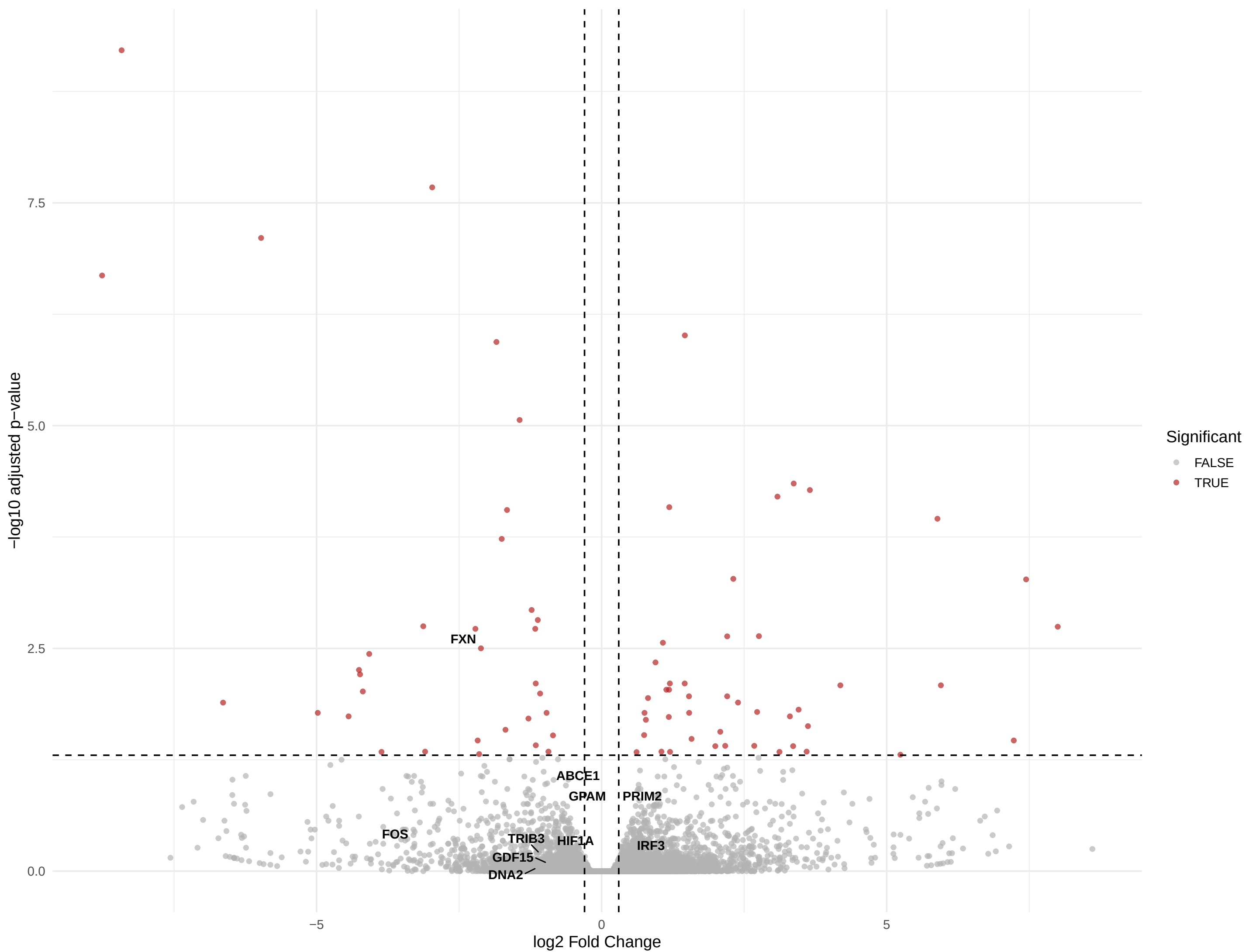
Volcano (genes of interest) – fibro control_vs_FA FA vs control
