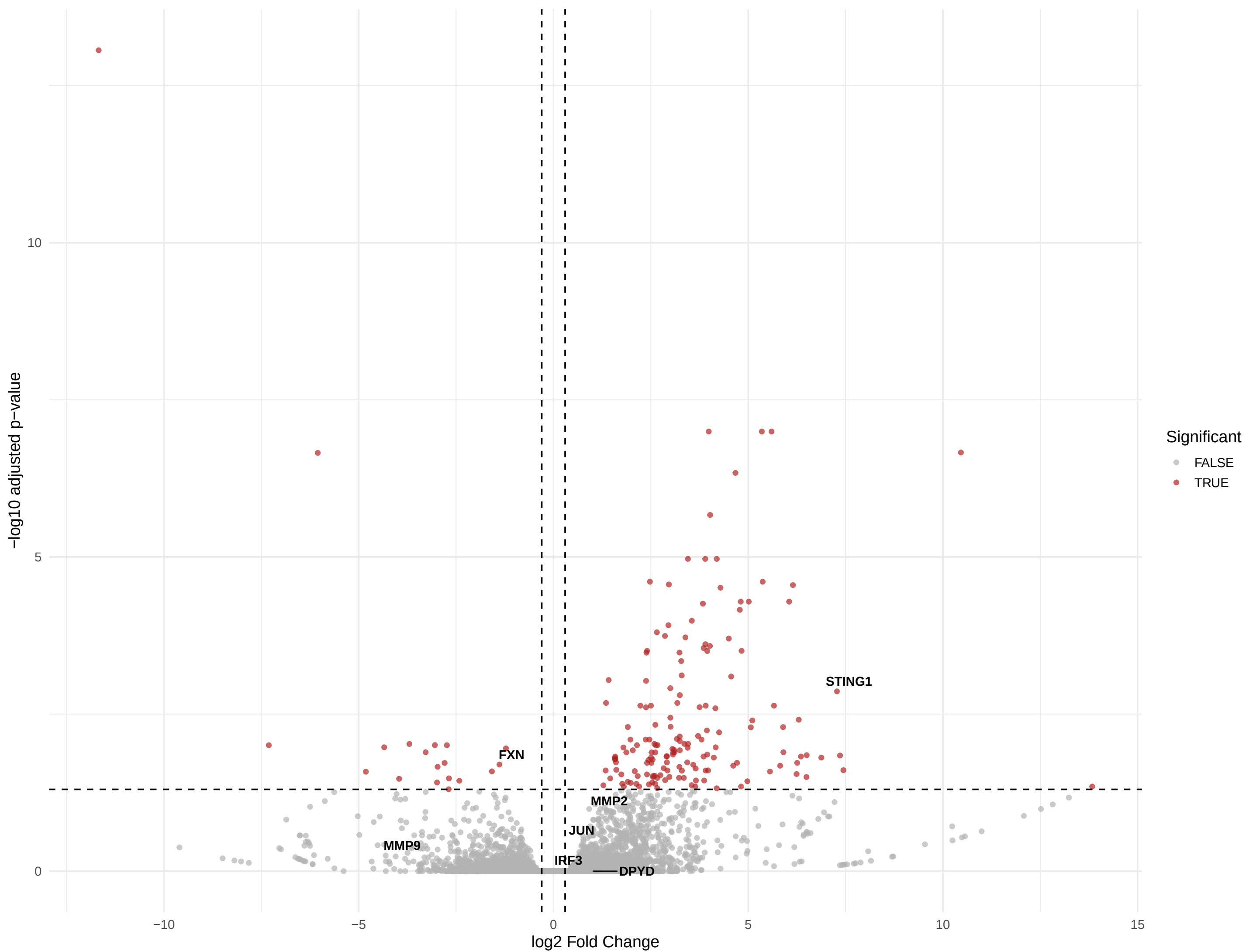
Volcano (genes of interest) – iNeurons control_vs_FA FA vs control
