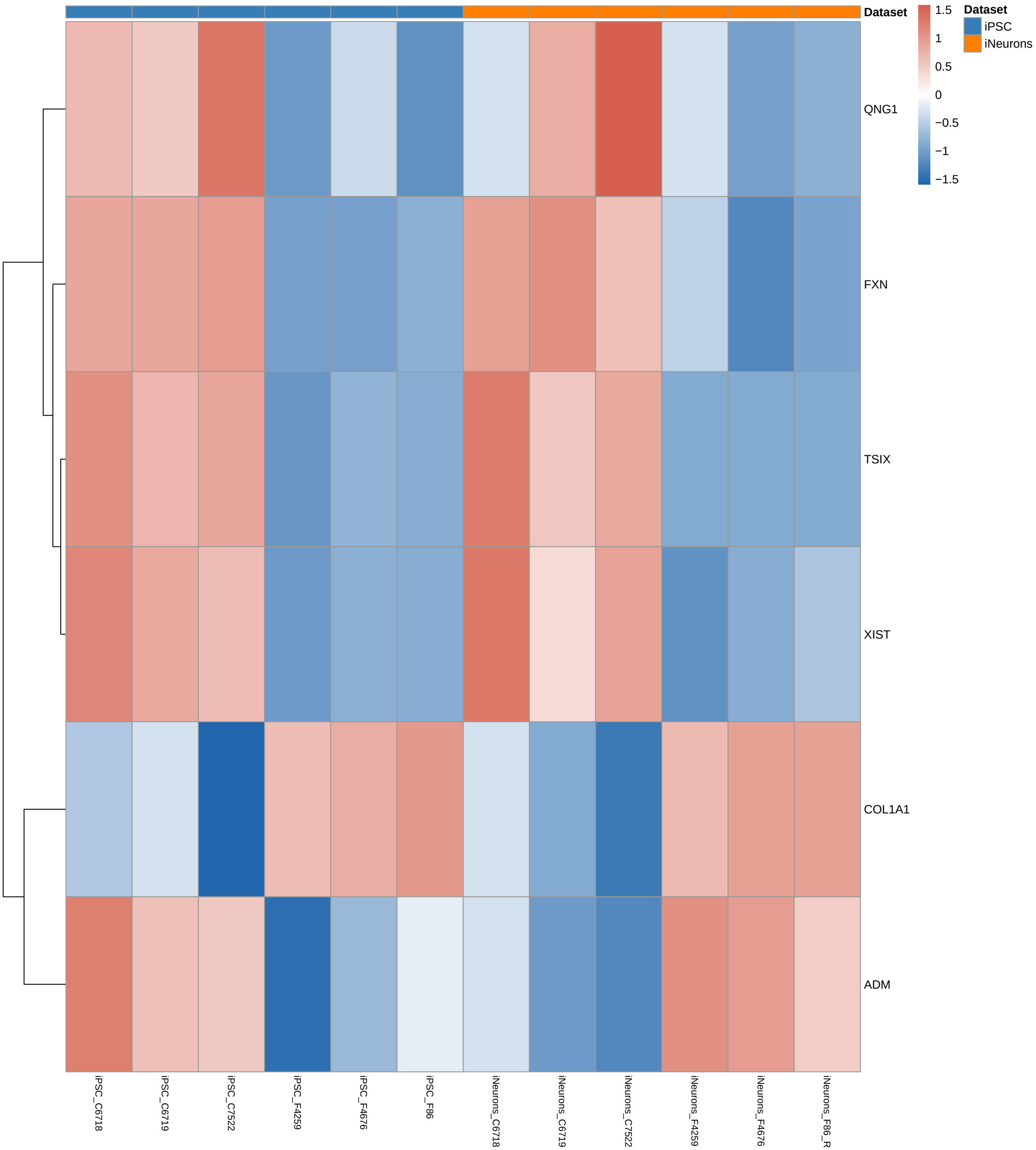
Shared DEGs (z-scored VST) control_vs_FA | iPSC || iNeurons
