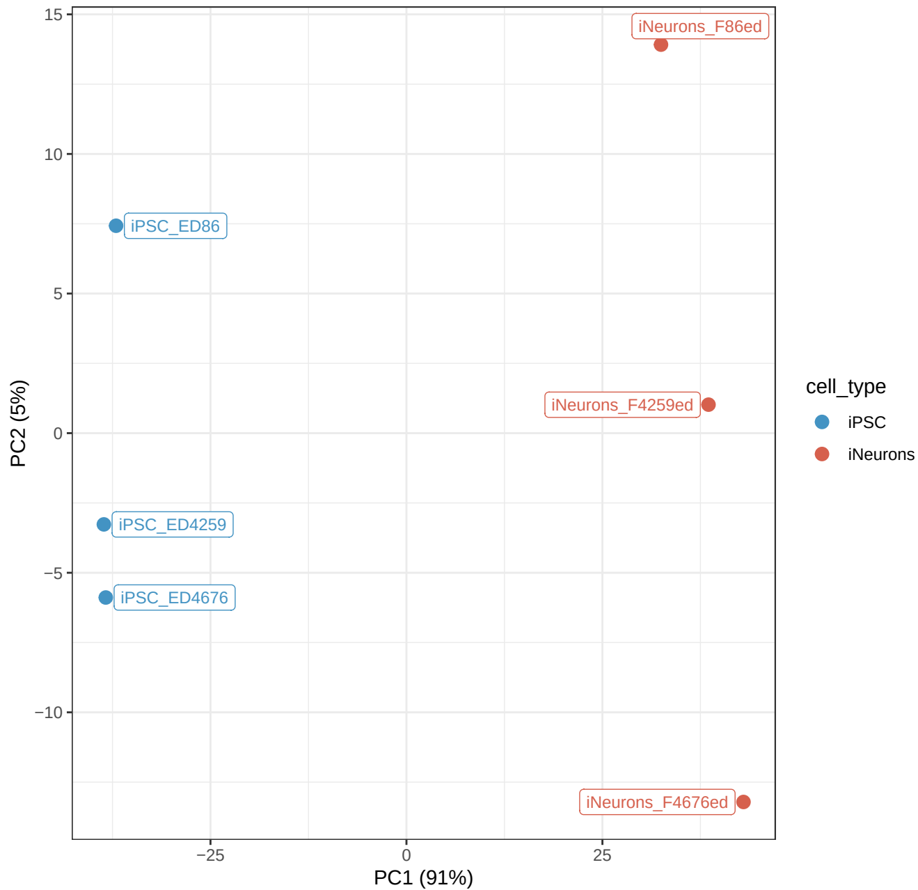
PCA iPSC vs iNeurons FA_edited [ENSG]
