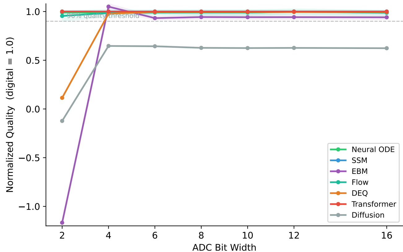
ADC Precision Tradeoff Quality at fixed mismatch \sigma=0.05 (50 trials per point)
