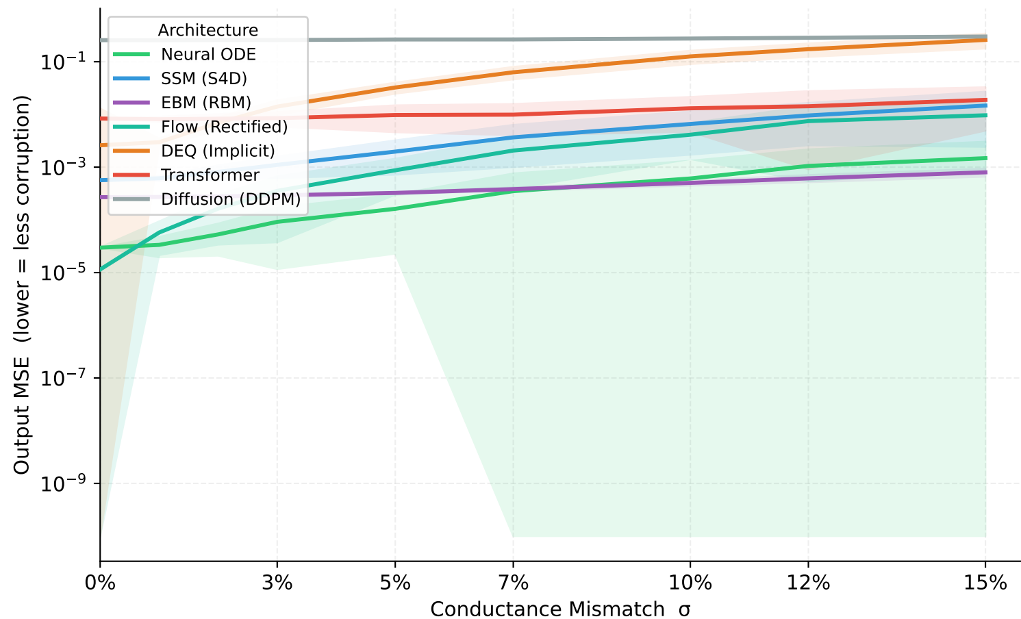
Output Corruption Under Analog Mismatch MSE between digital and analog outputs (50-200 Monte Carlo trials)
