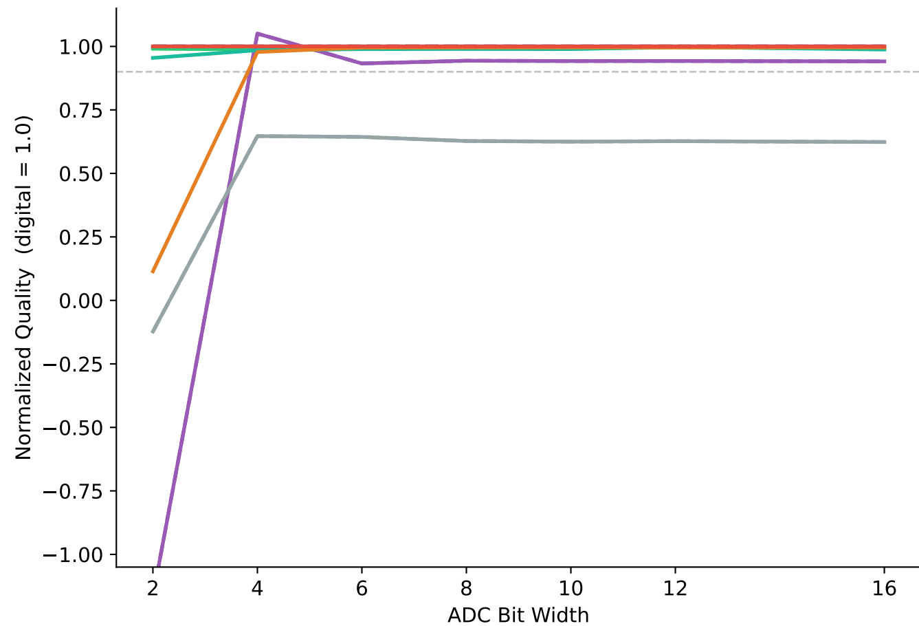
Conservative vs. Full-Analog ADC Precision ( \sigma=0.05 )
