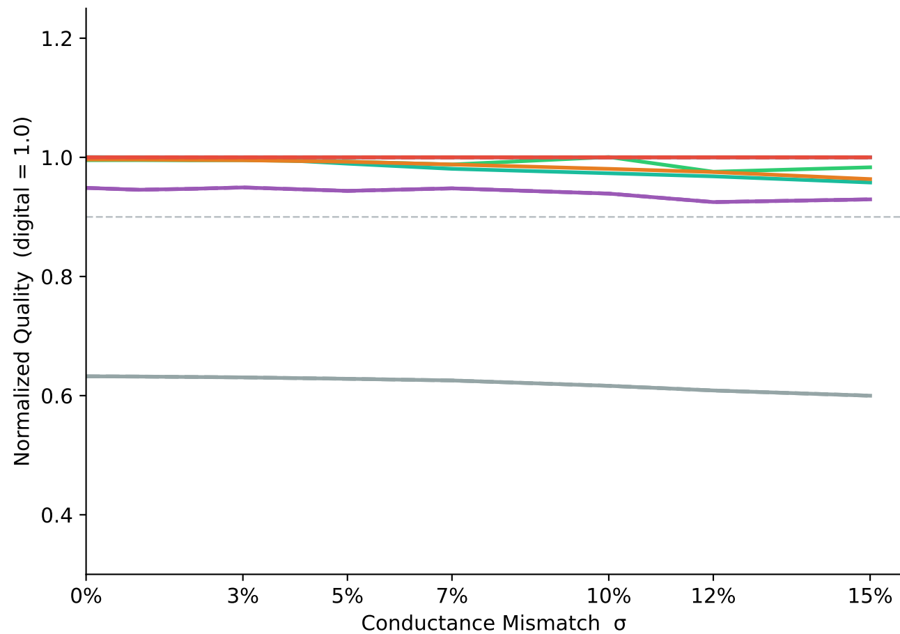
Conservative vs. Full-Analog Mismatch Tolerance
