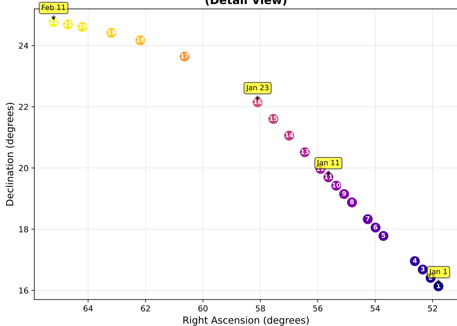
Piazzini's 22 Observations of Ceres (Detail View)
