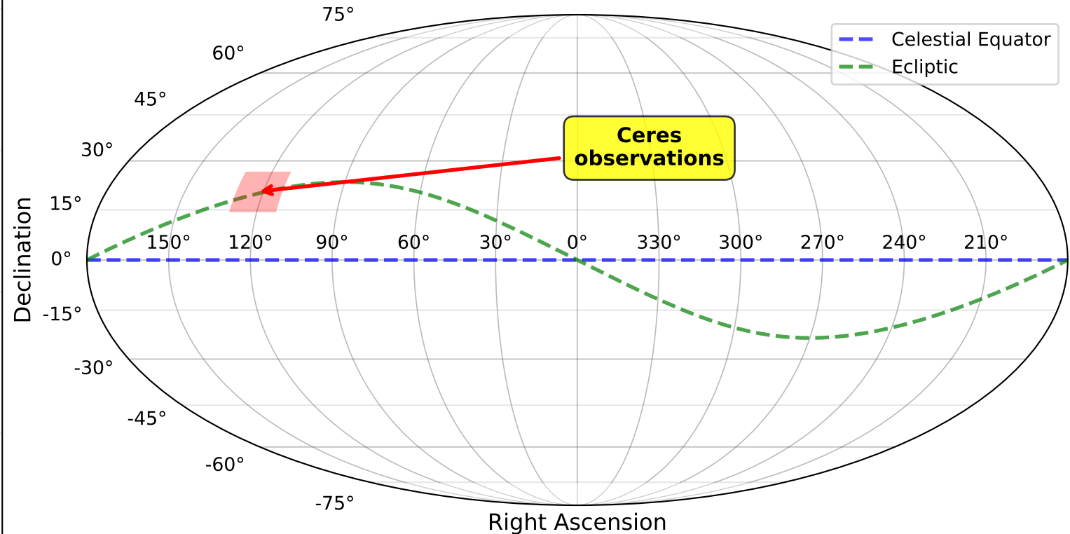
Full Sky Context - Ceres Observations in Red
