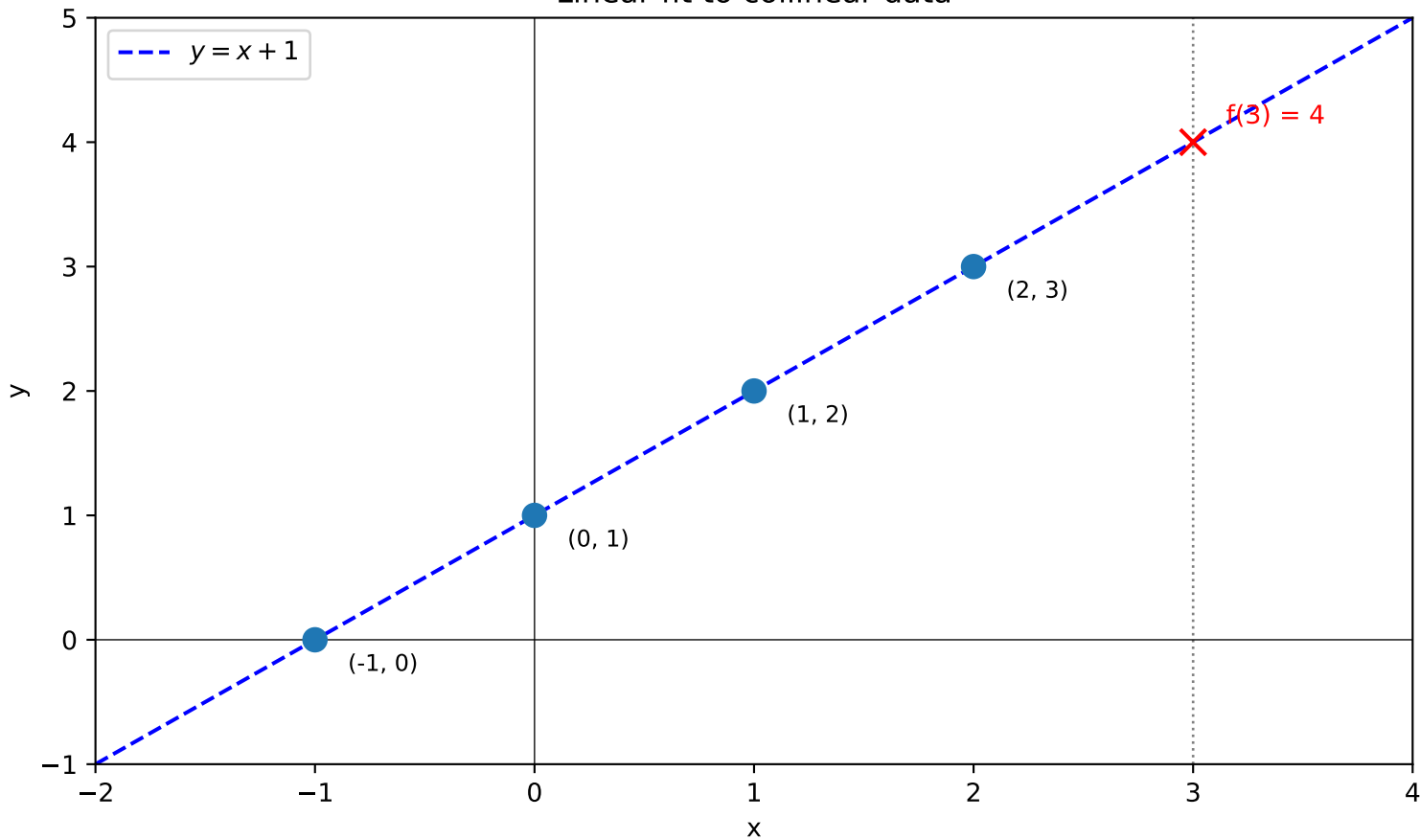
Linear fit to collinear data
