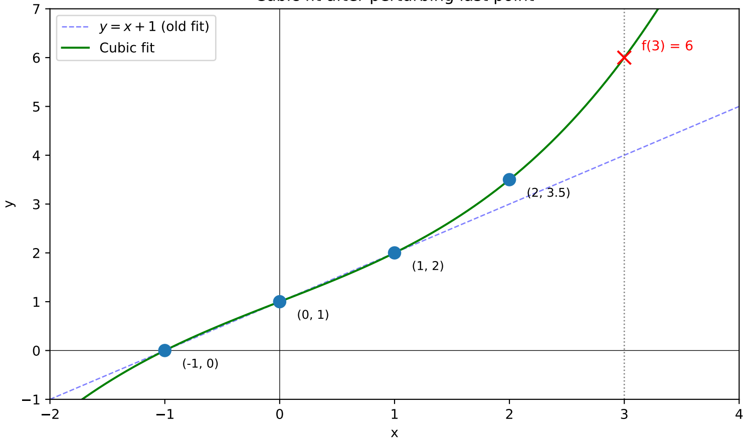
Cubic fit after perturbing last point
