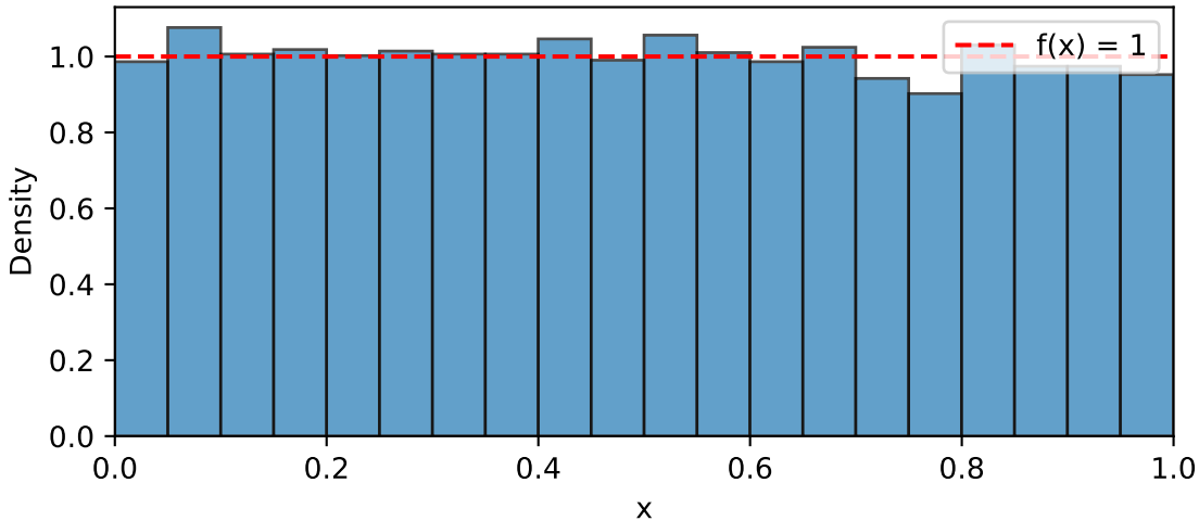
Histogram of 10,000 Uniform Samples
