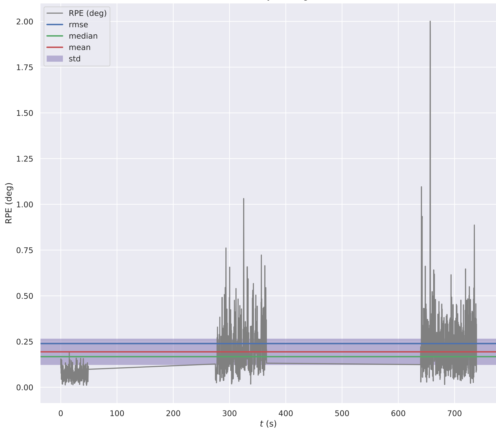
RPE w.r.t. rotation angle in degrees (deg) for \delta = 1 (frames) using consecutive pairs (with SE(3) Umeyama alignment)
