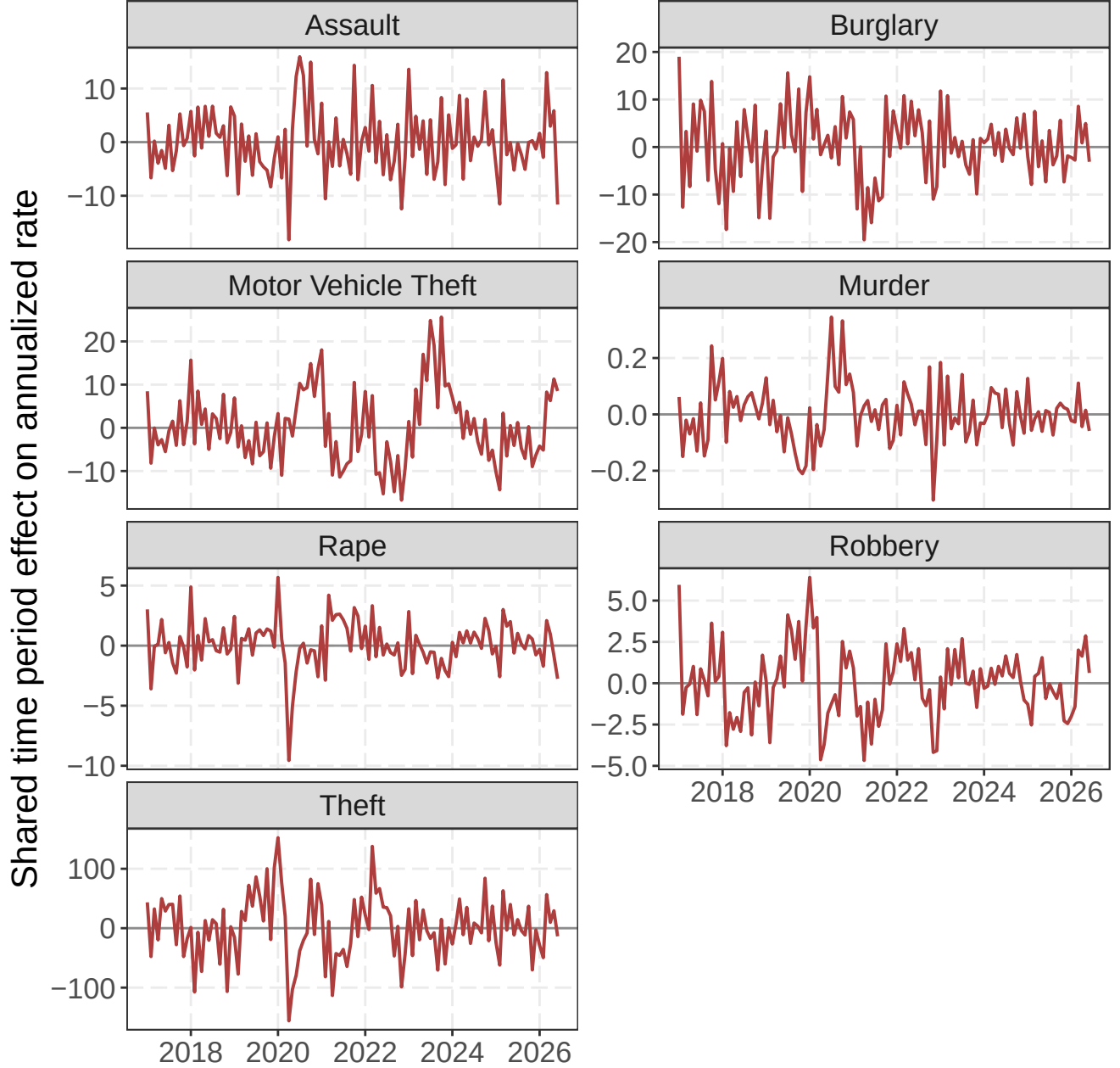
Figure 3: Fitted shared time-period random effect for each offense, transformed to its change in the annualized global rate. Positive values are time-period departures above the global trend-plus-seasonal curve; negative values are departures below it. Panels use offense-specific vertical scales.
