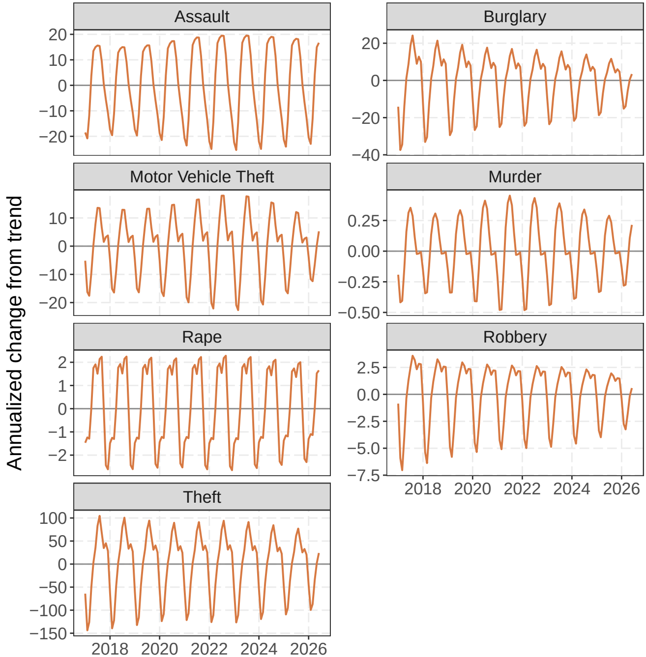
Figure 2: Estimated global cyclic seasonal departure for each offense on the annualized rate scale. Zero denotes the corresponding global trend; positive values indicate months above that trend and negative values indicate months below it. Panels use offense-specific vertical scales.
