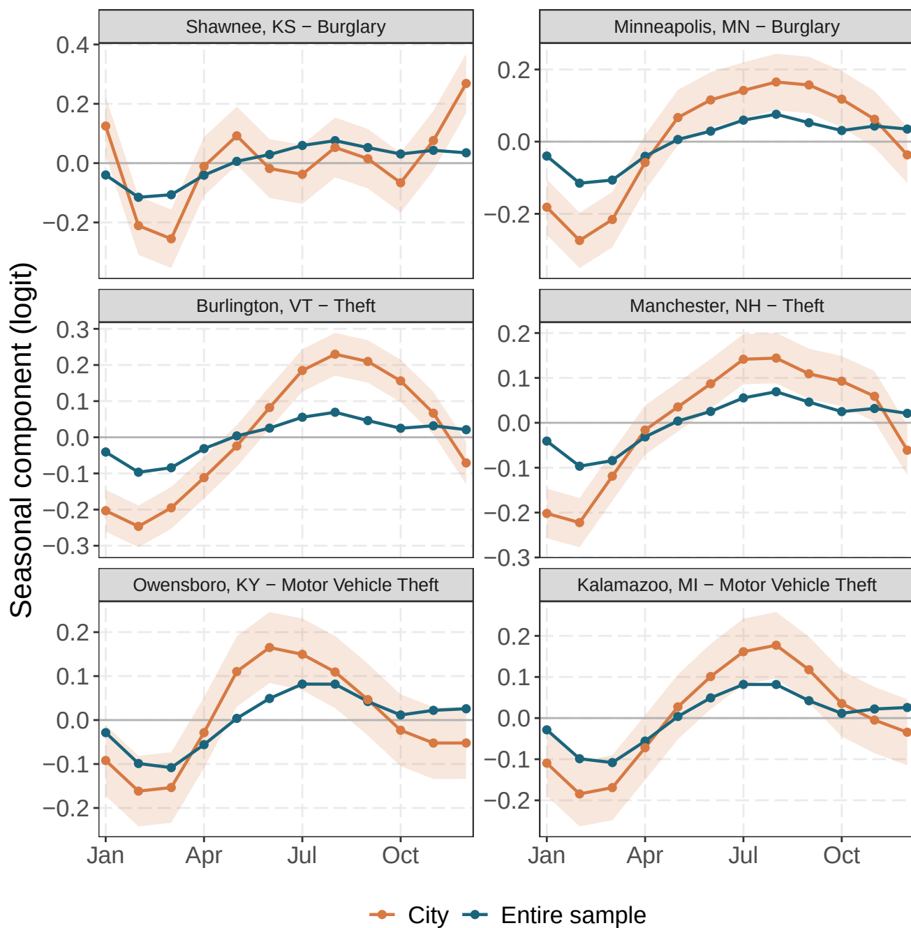
Figure 11: The two most unusual city-specific seasonal patterns within burglary, theft, and motor vehicle theft. Curves show the global and city-specific Fourier seasonal components over month of year on the logit scale; intercepts, trends, and residual terms are excluded. Shading gives approximate 95% pointwise conditional intervals for each city's seasonal deviation.
