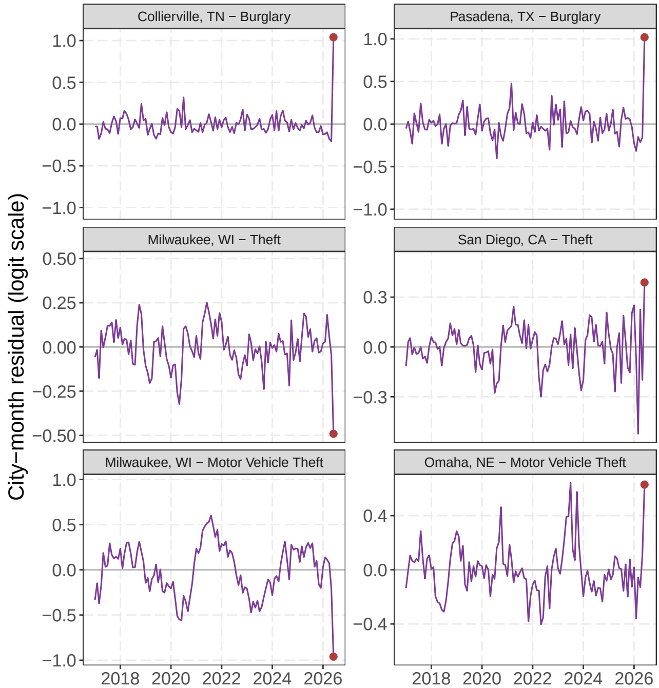
Figure 15: The two largest absolute fitted city-month residuals in the most recent month within burglary, theft, and motor vehicle theft. Lines provide each selected city’s full residual history for context; red points mark the latest month used for ranking. Panels are centered at zero and use city-specific symmetric vertical scales.
