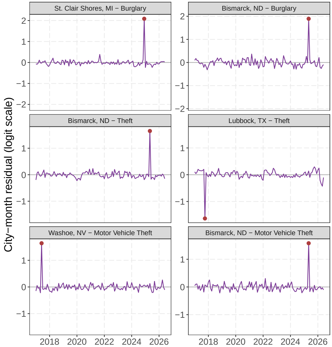
Figure 13: The two cities with the largest absolute fitted city-month residuals within burglary, theft, and motor vehicle theft. Lines show the observation-level city-month effect over time; red points mark the month used for ranking. Panels are centered at zero and use city-specific symmetric vertical scales.
