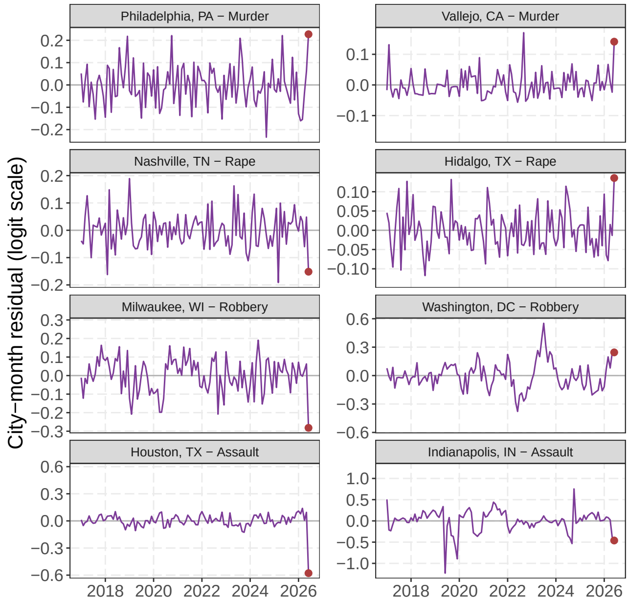
Figure 14: The two largest absolute fitted city-month residuals in the most recent month within murder, rape, robbery, and assault. Lines provide each selected city’s full residual history for context; red points mark the latest month used for ranking. Panels are centered at zero and use city-specific symmetric vertical scales.
