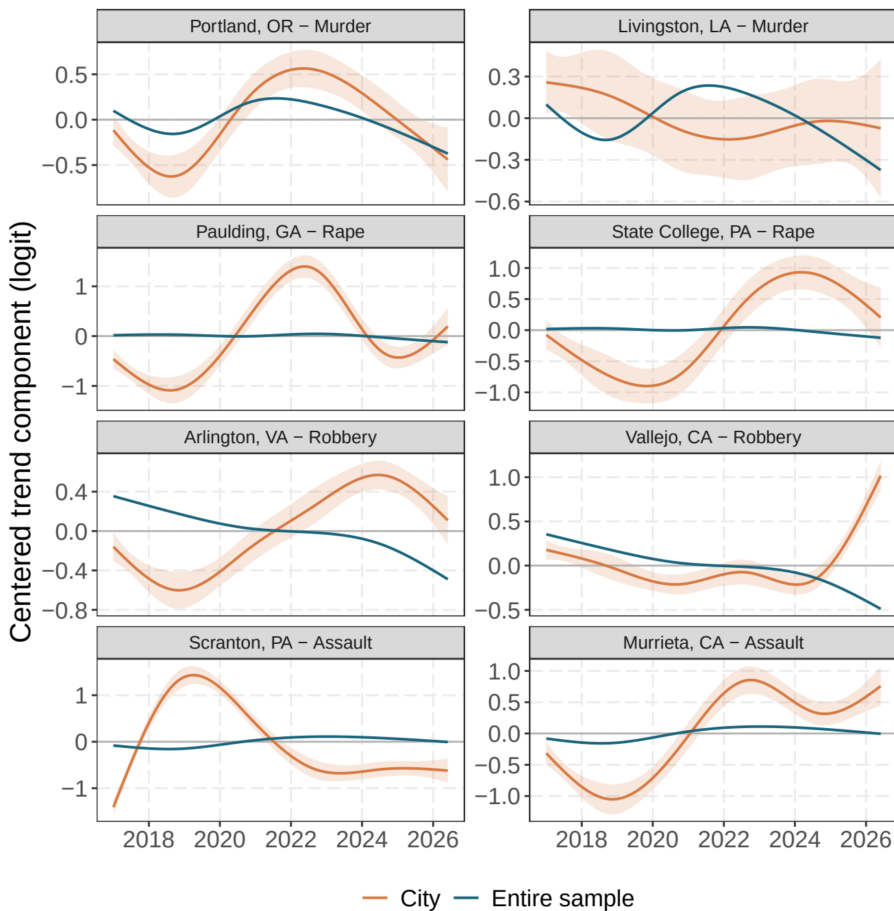
Figure 8: The two most unusual city-specific trends within murder, rape, robbery, and assault. City and global spline trends are centered separately, removing intercept differences. Selection uses within-offense robust standardized RMS trend departure; seasonal and residual terms are excluded. Shading gives approximate 95% pointwise conditional intervals for each city's trend deviation.
