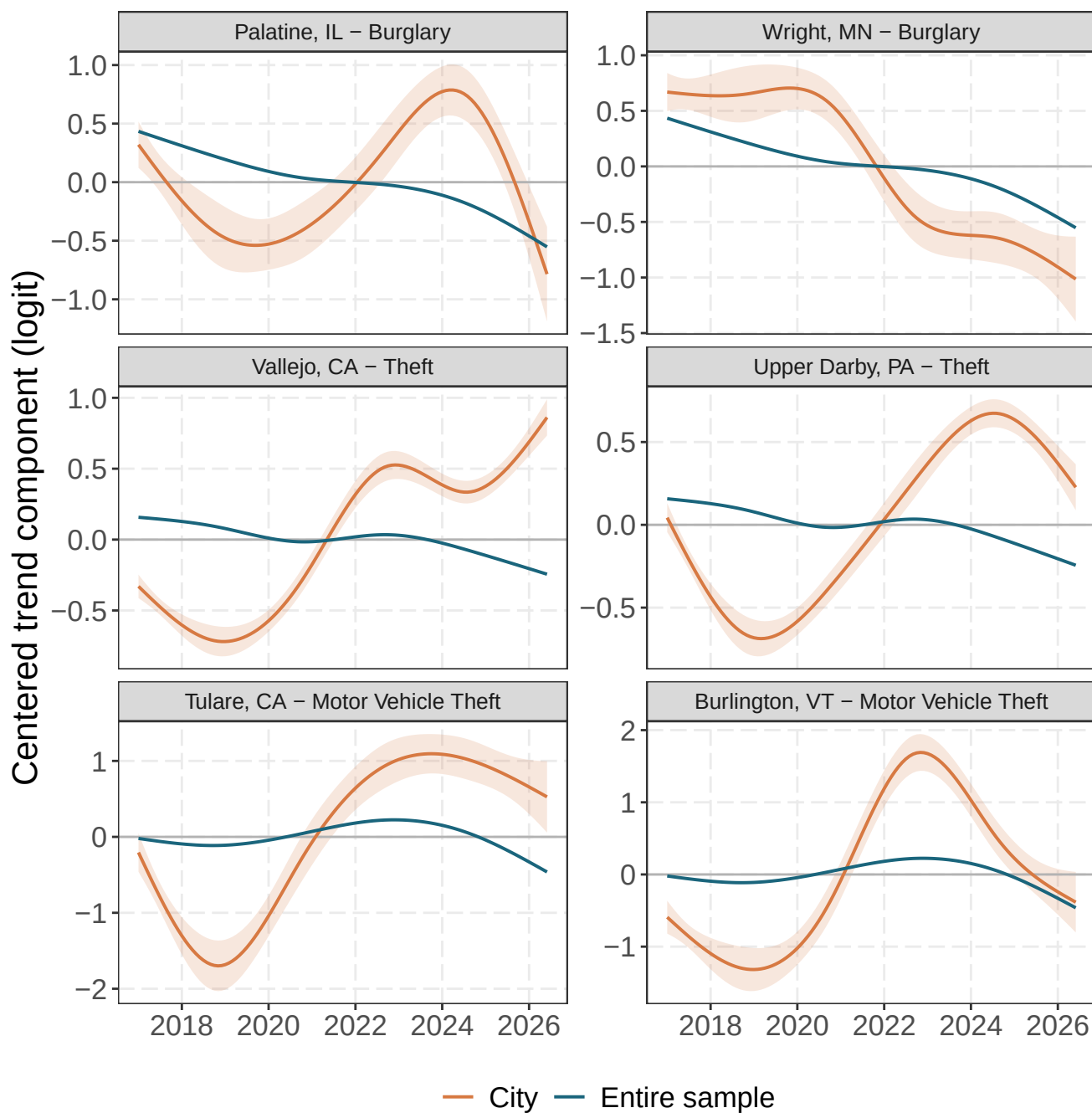
Figure 9: The two most unusual city-specific trends within burglary, theft, and motor vehicle theft. City and global spline trends are centered separately, removing intercept differences. Selection uses within-offense robust standardized RMS trend departure; seasonal and residual terms are excluded. Shading gives approximate 95% pointwise conditional intervals for each city's trend deviation.
