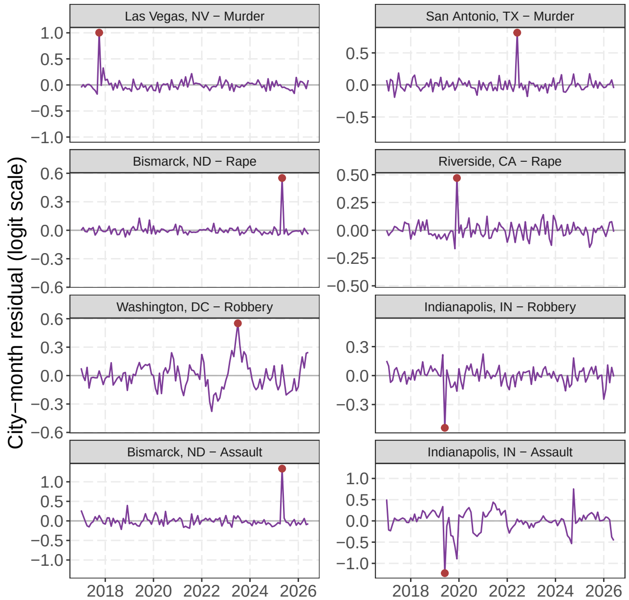
Figure 12: The two cities with the largest absolute fitted city-month residuals within murder, rape, robbery, and assault. Lines show the observation-level city-month effect over time; red points mark the month used for ranking. Panels are centered at zero and use city-specific symmetric vertical scales.
