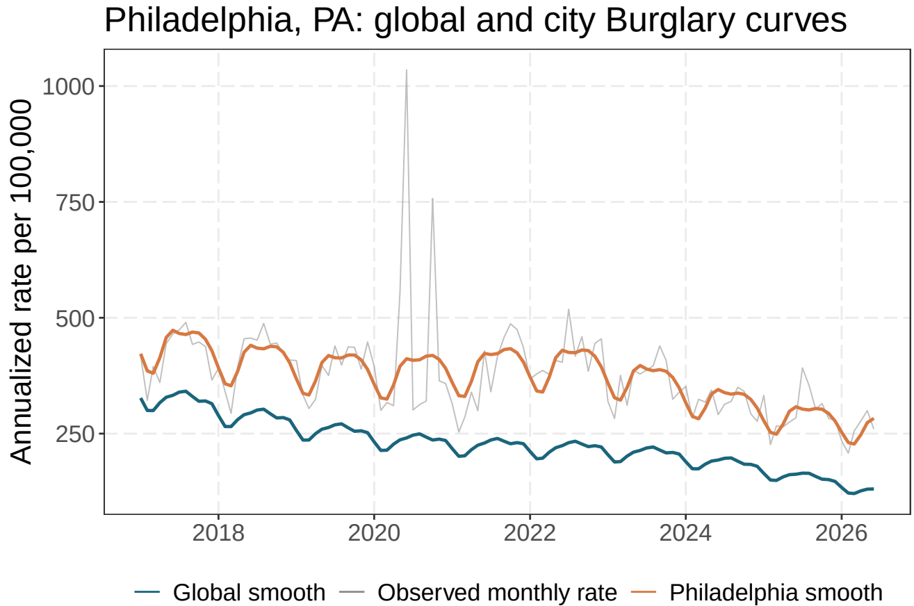
Figure 6: Philadelphia burglary rates: reported monthly observations, the global structural curve, and Philadelphia's fitted city curve. The pronounced May, June, and October 2020 observations come directly from the RTCI source counts; the smooth curves exclude shared time-period and city-month residual effects.
