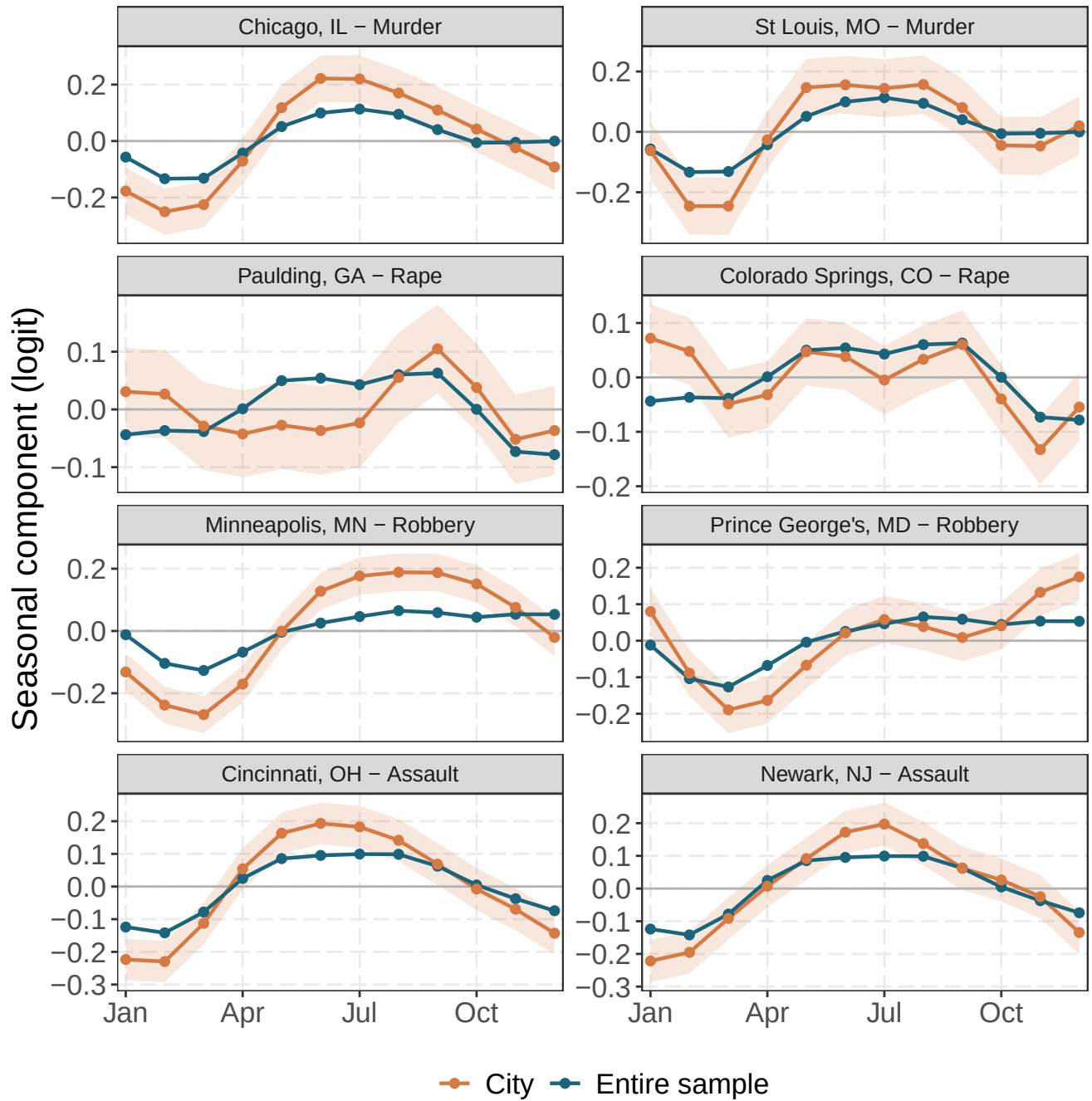
Figure 10: The two most unusual city-specific seasonal patterns within murder, rape, robbery, and assault. Curves show the global and city-specific Fourier seasonal components over month of year on the logit scale; intercepts, trends, and residual terms are excluded. Shading gives approximate 95% pointwise conditional intervals for each city's seasonal deviation.
