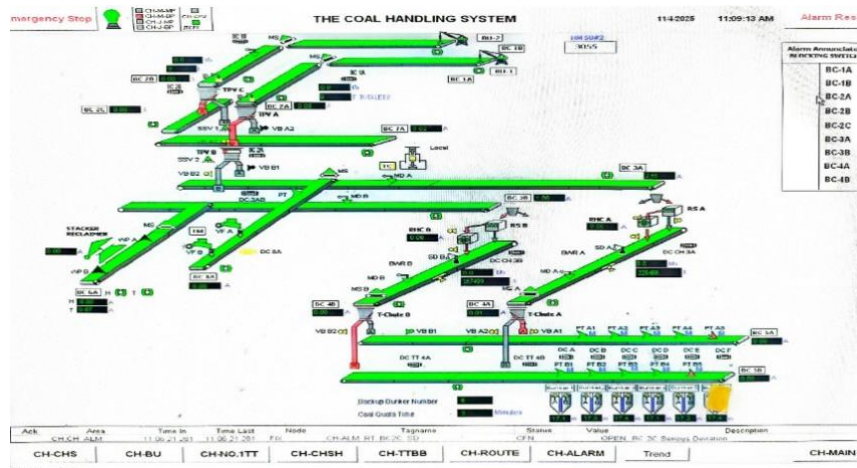
Gambar 3. 4 Coal Handling System
