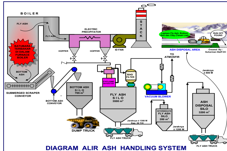
Gambar 3. 5 Ash Handling System
