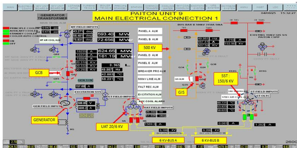
Gambar 5. 1 Main Electrical Connection
