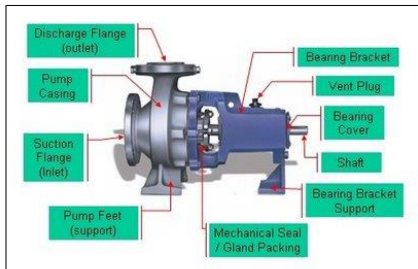
Gambar 4.2 Komponen Condensate Transfer Pump
