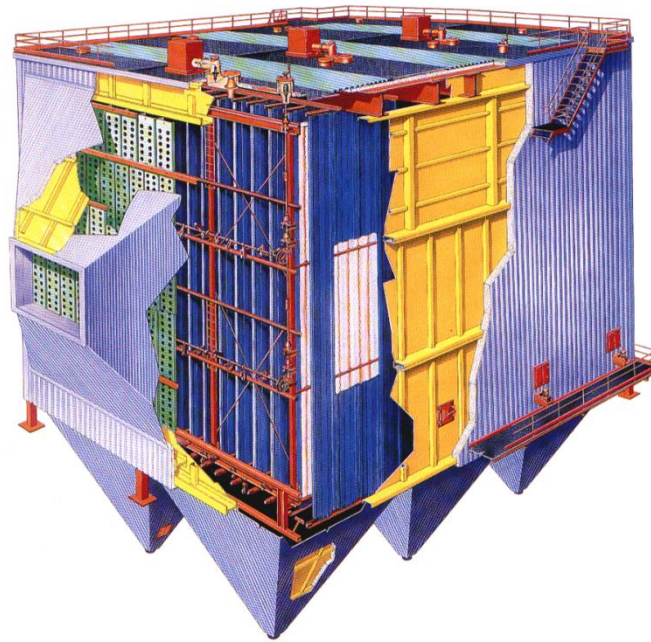
Gambar 3. 5 Electrostatic Precipitator
