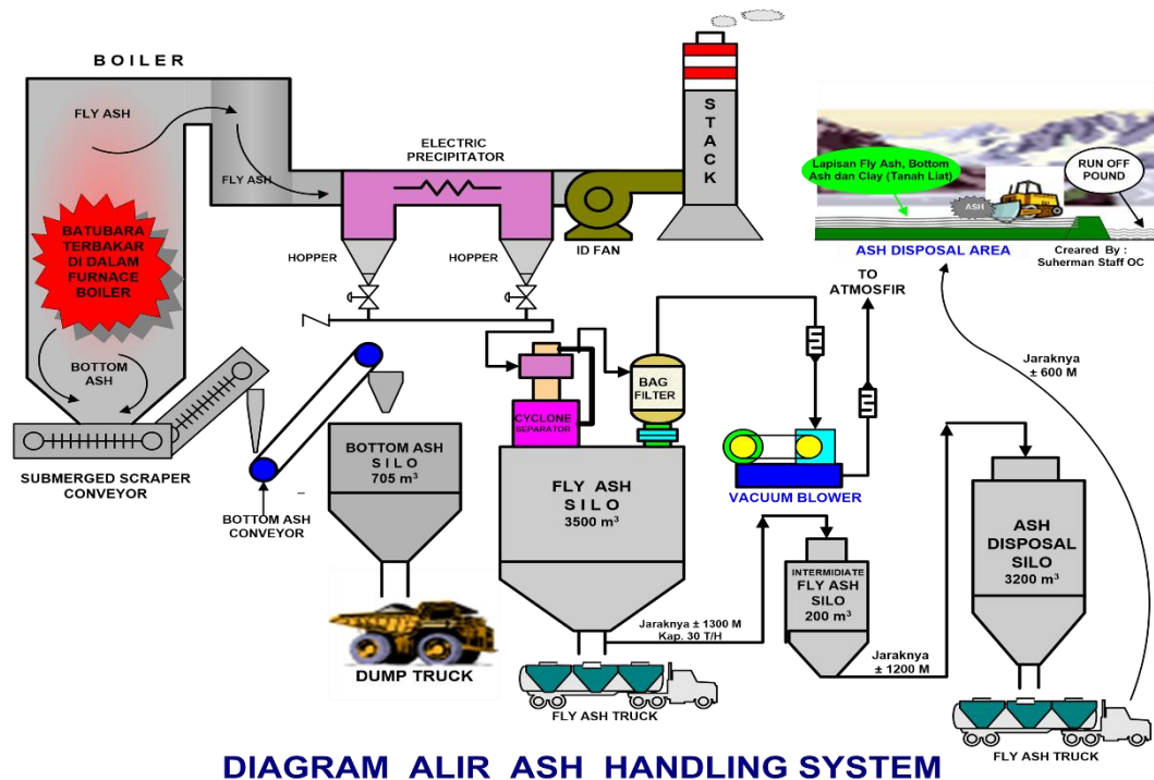
Gambar 3. 4 Sistem Penanganan Abu Batu Bara (Ash Handling)
