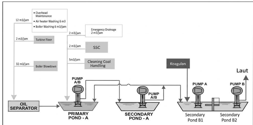
Gambar V. 1 PFD Metal Cleaning Waste Water Treatment Plant
