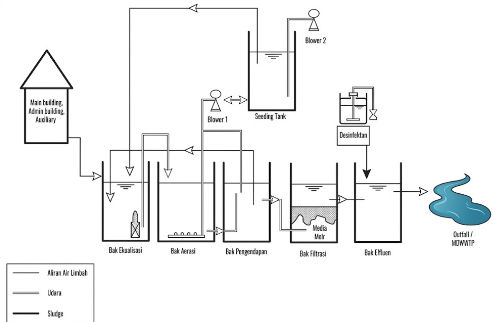
Gambar V. 5 PFD Pengolahan Air Limbah Sewage Treatment Plant
