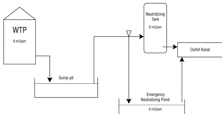
Gambar V. 2 PFD Pengolahan Air Limbah WTP
