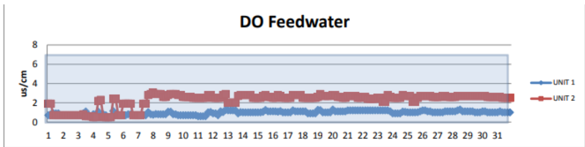
Gambar IV. 31 Grafik Dissolved Oxygen Feedwater
