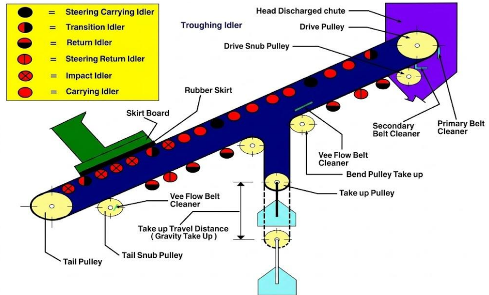
Gambar IV. 4 Conveyor System
