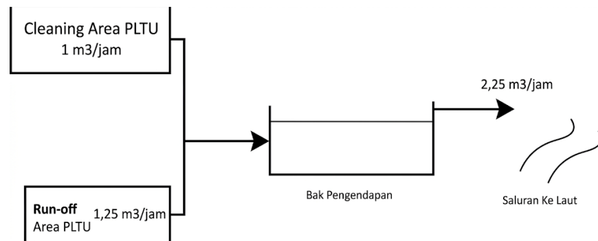
Gambar V. 4 PFD Pengolahan Limbah Drainase Oily Water
