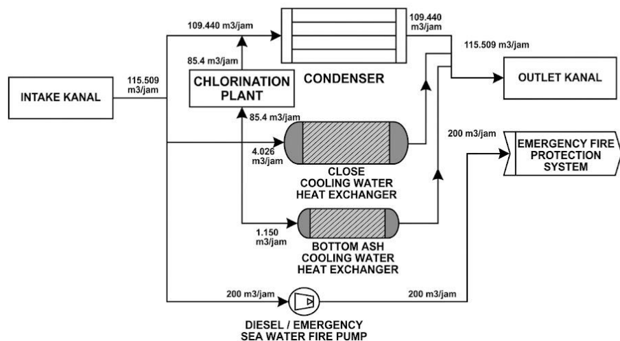
Gambar V. 3 PFD Pengolahan Limbah Air Pendingin
