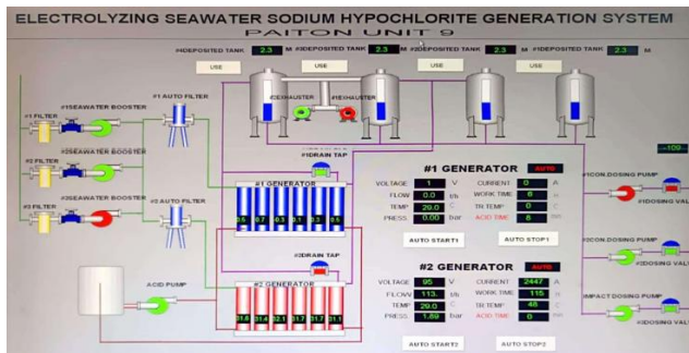
Gambar 3. 42 Sistem Chlorine Plant Sumber : PT.PLN Nusantara Power UP Paiton
