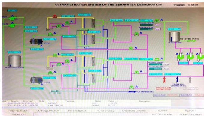
Gambar 3. 18 Sistem Ultrafiltration
