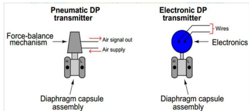
Gambar 3.7 Bagian – bagian luar Diffrential Pressure Transmitter
