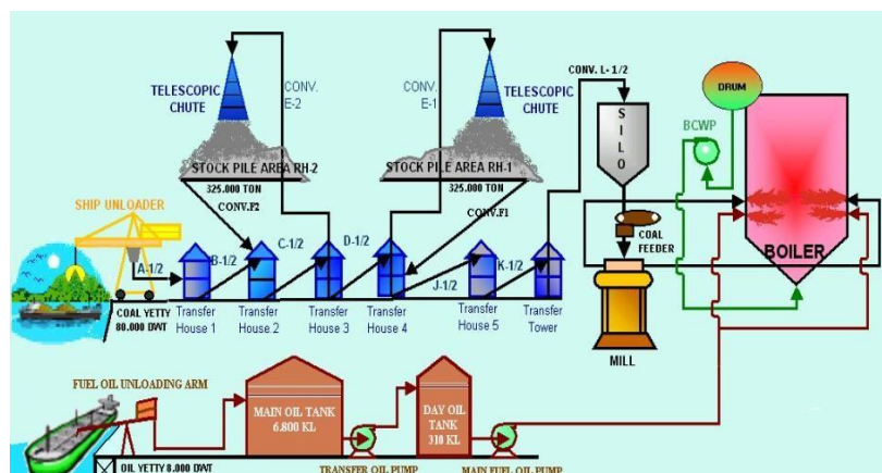
Gambar 2.9 Diagram alur Coal Handling System
