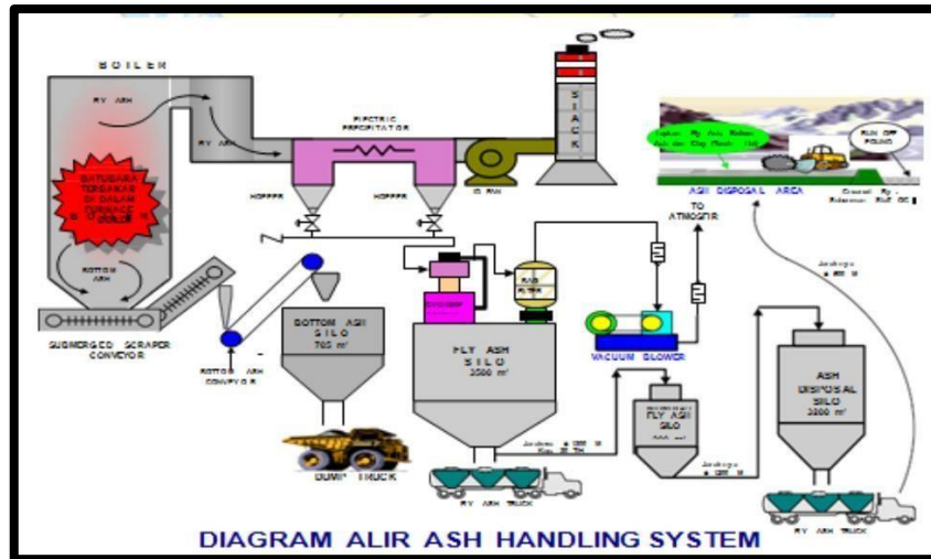
Gambar 2.10 Diagram alur Ash Handling System
