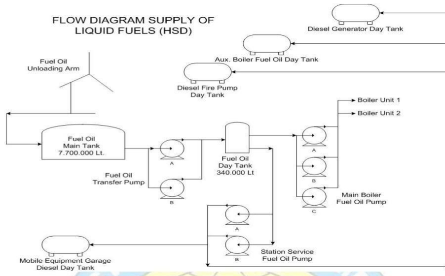
Gambar 2.14 Diagram alur Fuel Oil System
