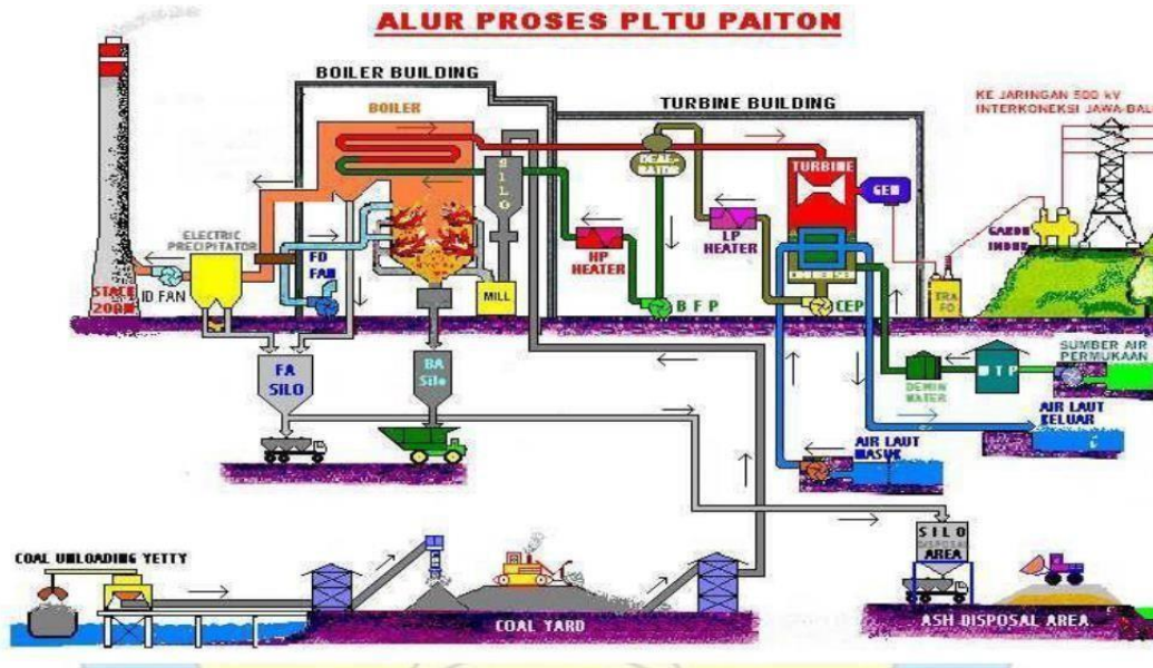
Gambar 2.6 Diagram alur proses PLTU Paiton
