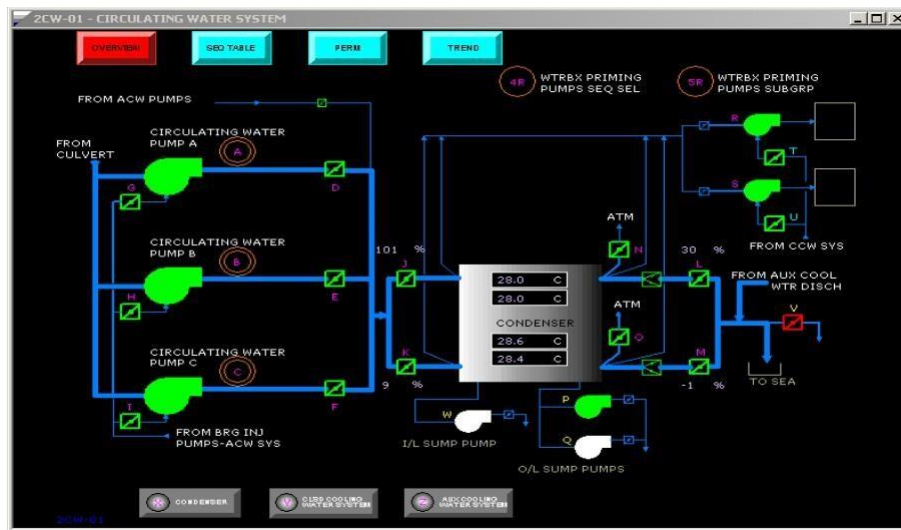
Gambar 2.13 Diagram alur Air Pendingin Condenser
