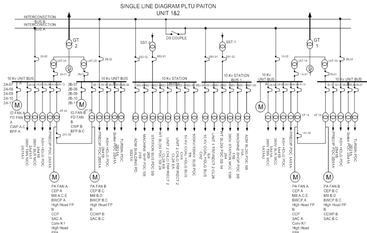
Gambar 2.15 Single Line Diagram PLTU Paiton
