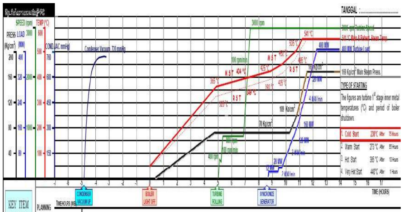
Gambar 2.32 Kurva Cold Star Turbin UP Paiton 1&2
