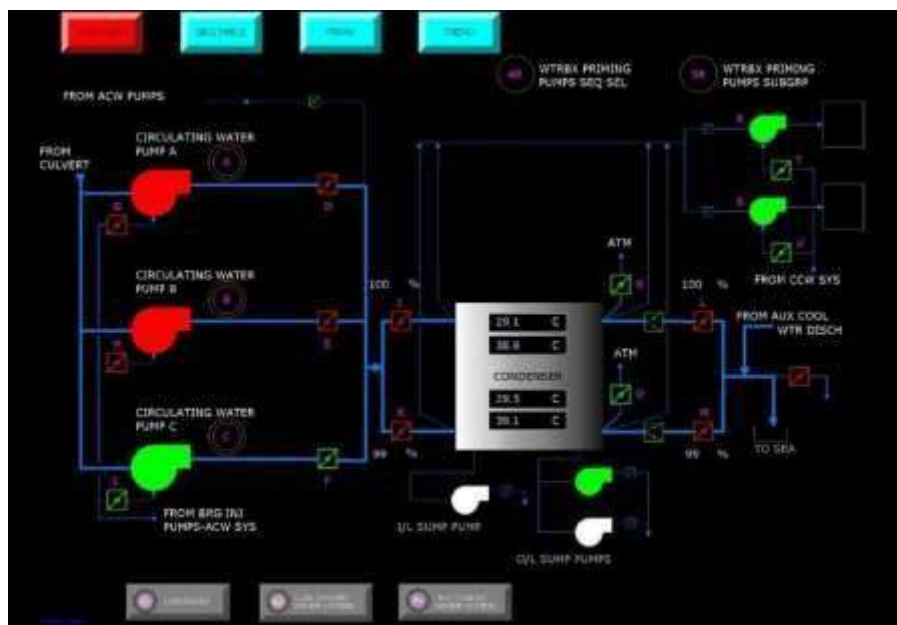
Gambar 2 24 Diagram Alir Condensor
