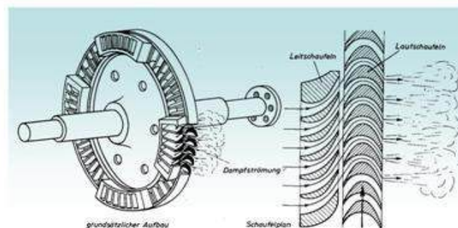
Gambar 2.29 Single Stage Turbin
