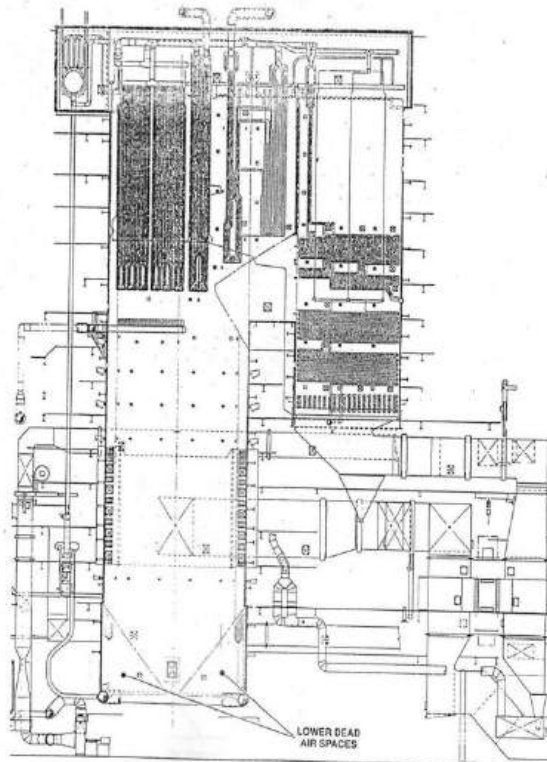
Gambar 2.26 Penampang Boiler
