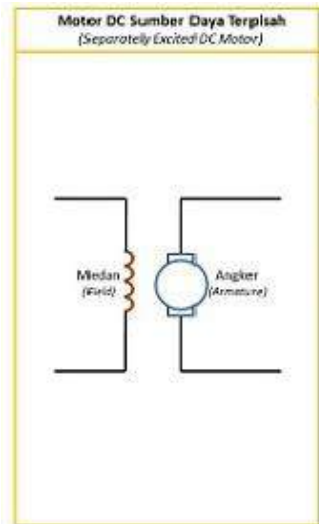
Gambar 3.1 Motor DC Separately Excited
