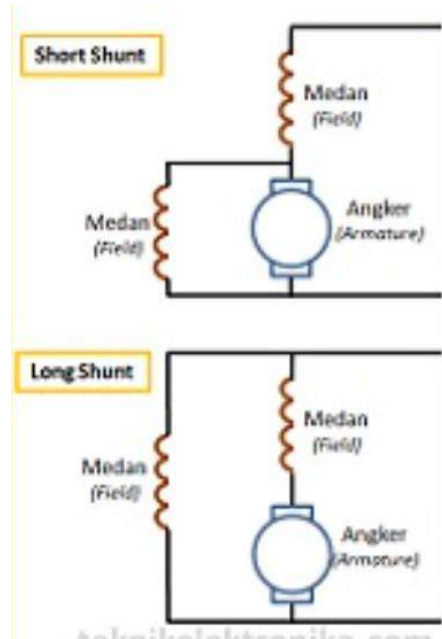
Gambar 3 4 Compound DC Motor
