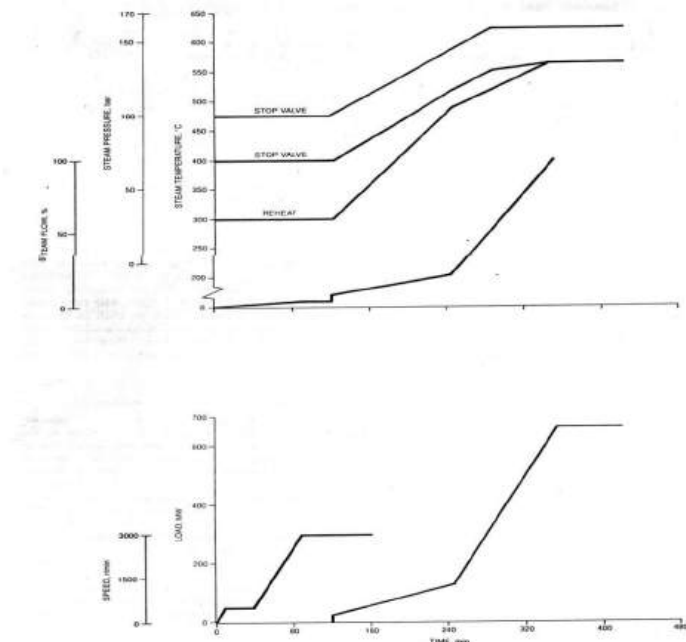
Gambar 2.31 Kurva Start UP Turbin
