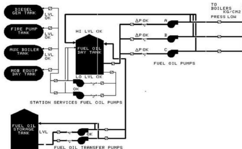
Gambar 2.18 Flow Diagram Fuel Oil System
