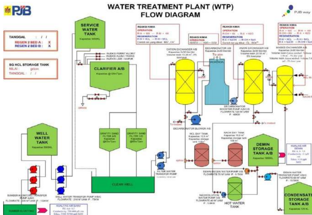
Gambar 2 23 Siklus Water Treatment Plant
