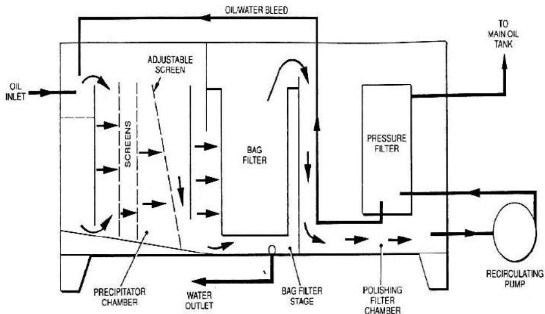
Gambar 2.30 Oil Conditioning Turbines
