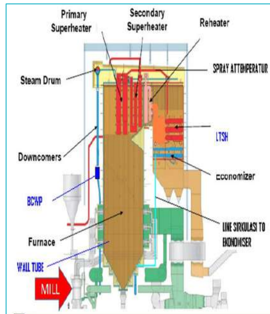
Gambar:3.2 Boiler
