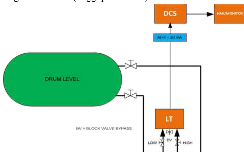
Gambar 5.6 Instalasi level transmitter
