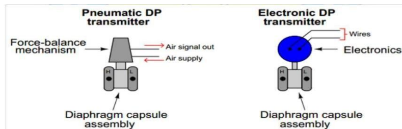
Gambar 3.3 Baqian – baqian luar Diffrential Pressure Transmitter
