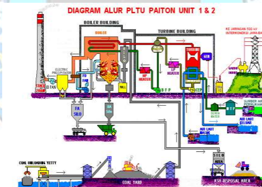
Gambar 0.10 Diagram Alur PLTU Paiton Unit 1&2
