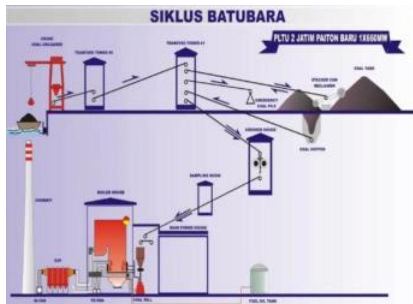
Gambar 3.14 Sistem Penanganan Batu Bara PLTU PT. PLN Nusantara Power UP Paiton Sumber : PT. PLN Nusantara Power UP. Paiton
