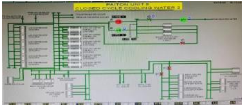
Gambar 3.101 Closed Cycle Cooling Water 2 PLTU PT. PLN Nusantara Power UP Paiton
