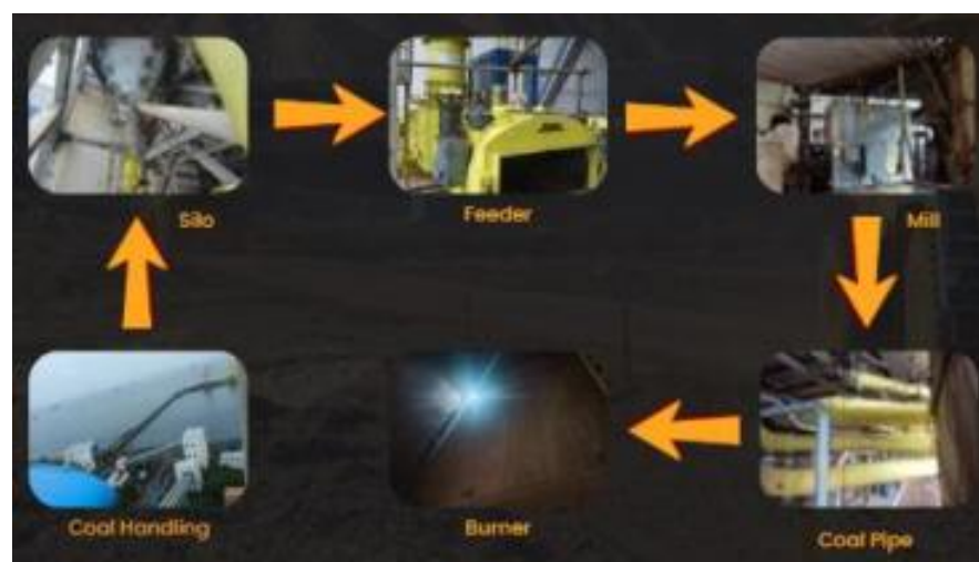
Gambar 3.15 Siklus Batu Bara PLTU PT. PLN NP UP Paiton Sumber : PT. PLN Nusantara Power UP. Paiton
