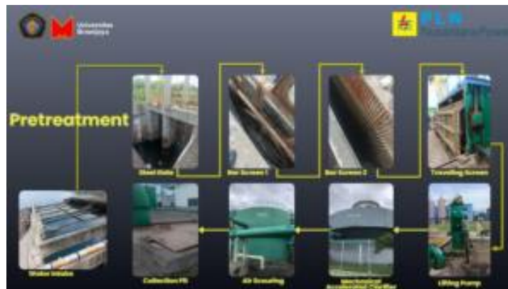
Gambar 3.19 Sistem Preatreatment PLTU PT. PLN Nusantara Power UP Paiton
