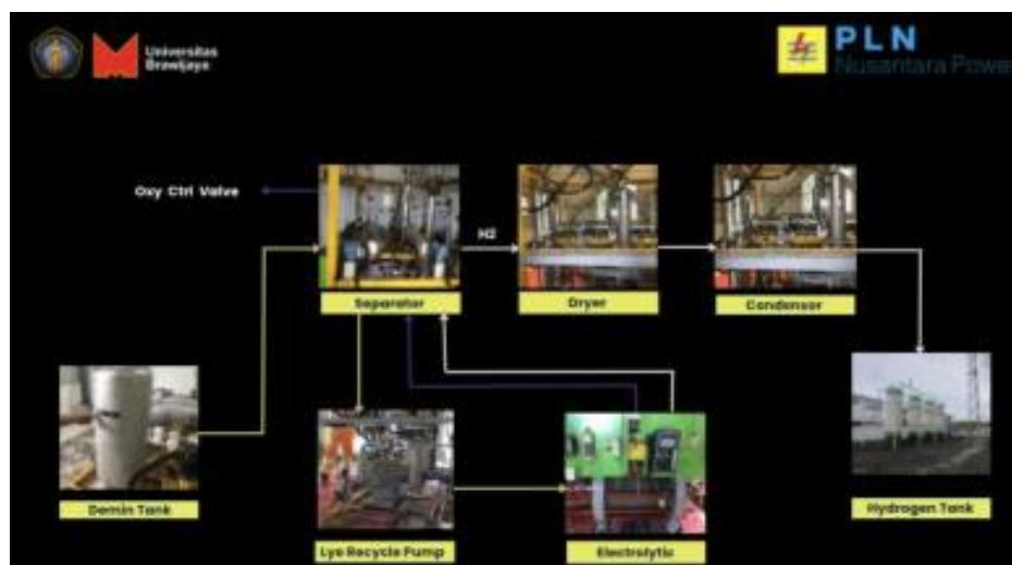
Gambar 3.53 Sistem Hydrogen PT. PLN Nusantara Power UP Paiton Sumber : PT. PLN Nusantara Power UP Paiton
