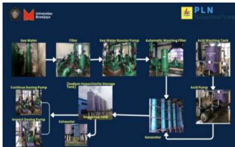
Gambar 3.60 Sistem Chlorine PT. PLN Nusantara Power UP Paiton Sumber : PT. PLN Nusantara Power UP Paiton
