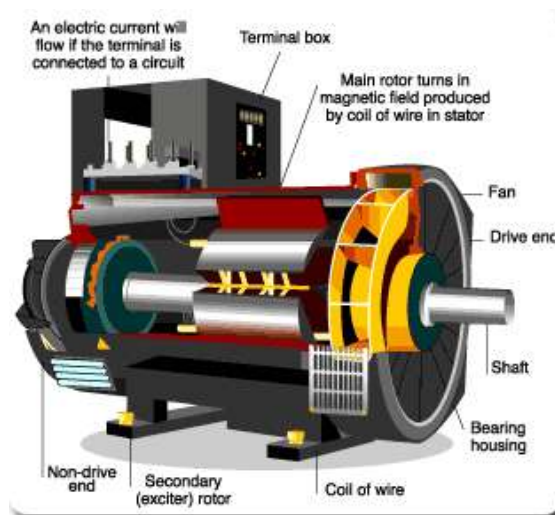
Gambar 2.1 Generator Sinkron
