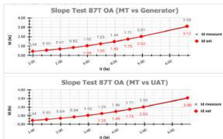
Gambar 4.12 Slope Test Proteksi Differensial 87T (Sumber: Data PT PLN NP UP Paiton Unit 9)
