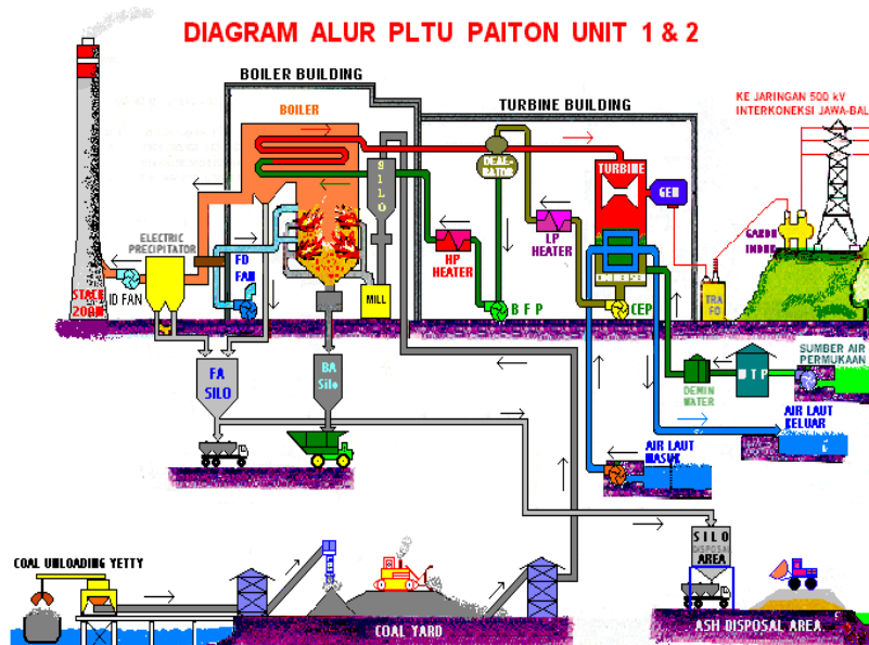
Gambar 2.10 Diagram Alur PLTU Paiton Unit 1&2
