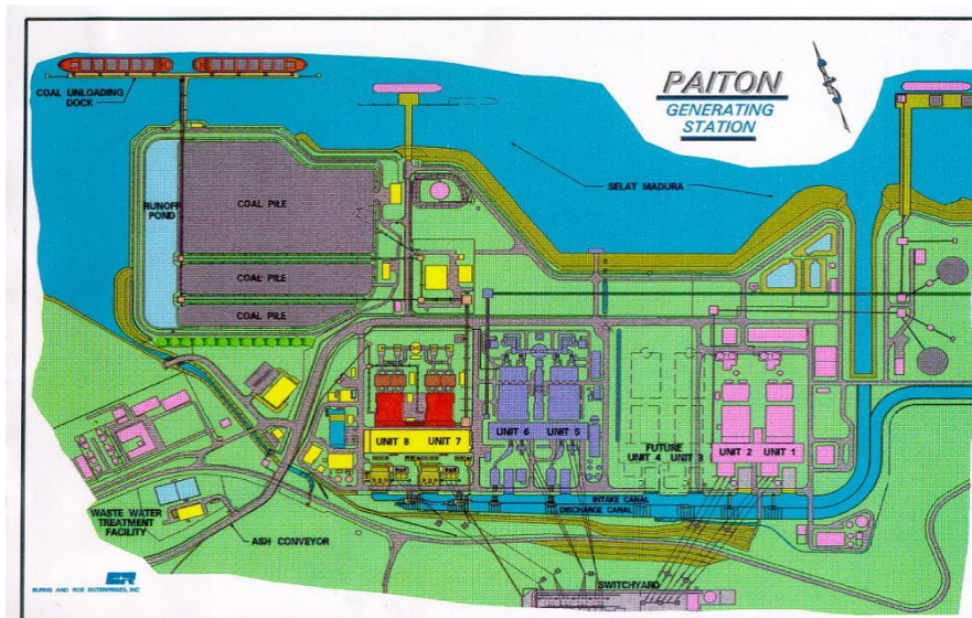
Gambar 2.6 Lay Out PLTU Paiton
