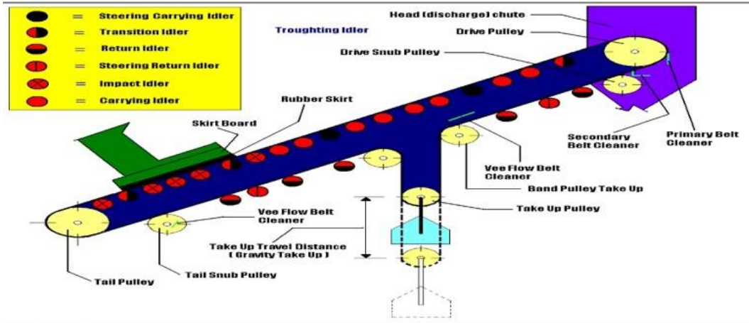
Gambar: 3.2.3 Gambar Conveyor System
