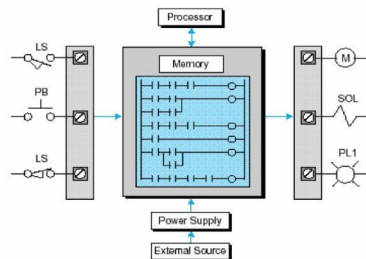
Gambar 5.3 Hirarki PLC
