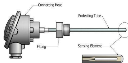
Gambar: 5.10 Thermocouple
