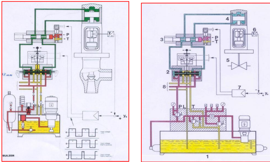
Gambar : 5.5.7 .Servo valve
