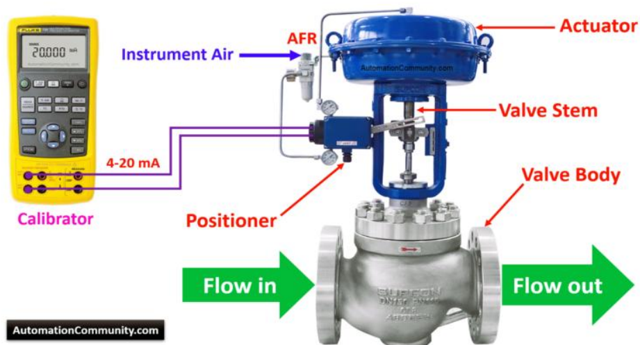
Gambar : 6.7 Kalibrasi Pneumatic Postioner
