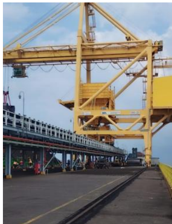
Gambar 3.20 Ship Unloader
