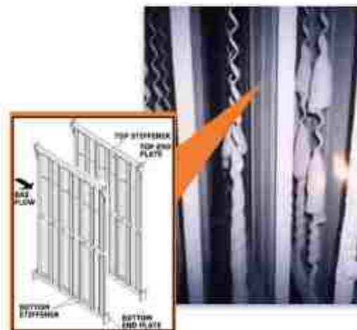
GAMBAR Collecting Electrode (CE)
