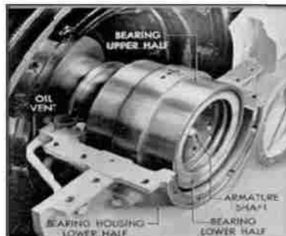
GAMBAR Rangkaian Bearing Generator
