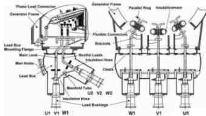
GAMBAR Generator Terminal
