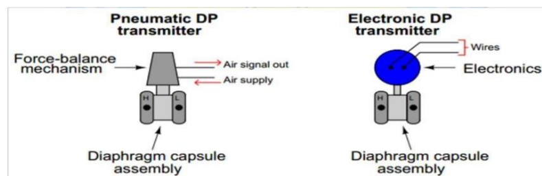
Gambar 3.3 Bagian – bagian luar Diffrential Pressure Transmitter
