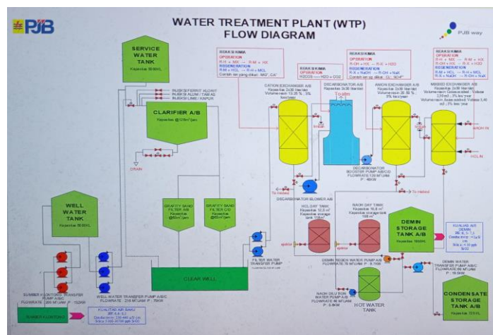
Gambar 2.11 Diagram alur Water Treatment Plant
