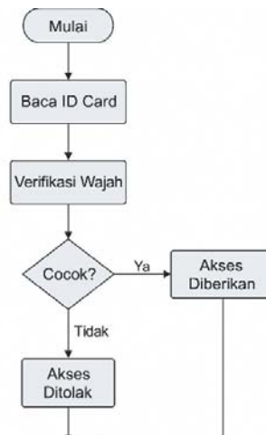
Gambar 4. 1. Alur Program
