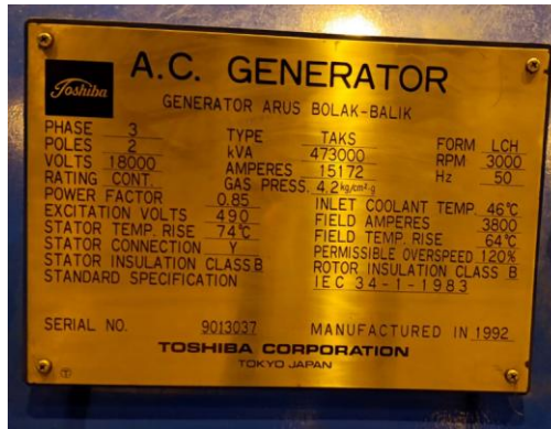
Gambar IV.2 Nameplate Generator PT PLN NP Paiton Unit 2
