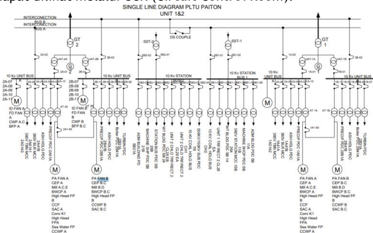
Gambar III.2 Single Line Diagram PLTU Paiton
