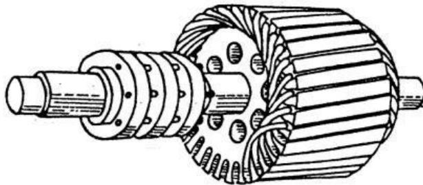
Gambar III.8 Gambar Rotor Lilit
