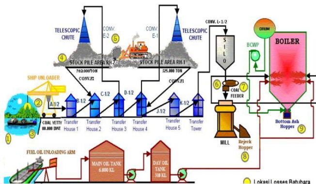
Gambar III.3 Diagram sistem penanganan batu bara
