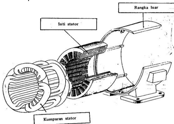
Gambar III.6 Struktur stator motor
