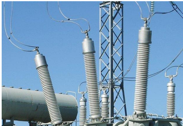
Gambar 2.9 Bushing Transformator
