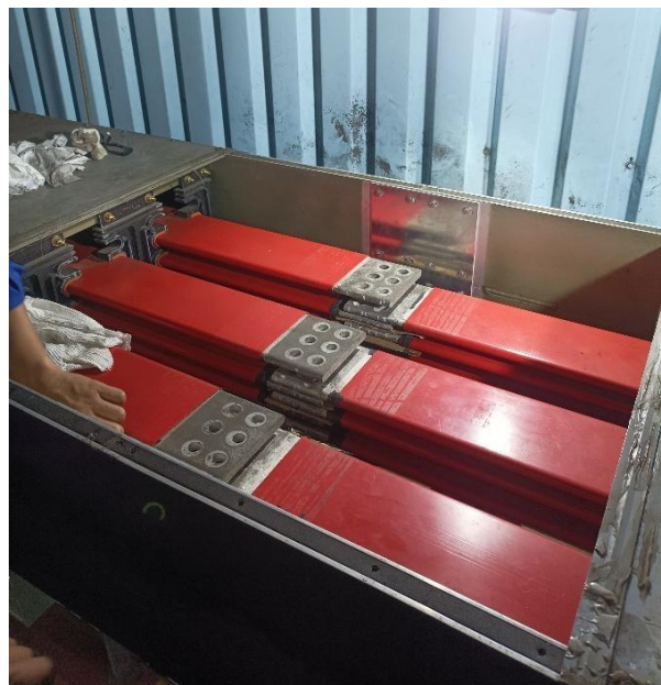
Gambar 2.8 Busbar 10 kv
