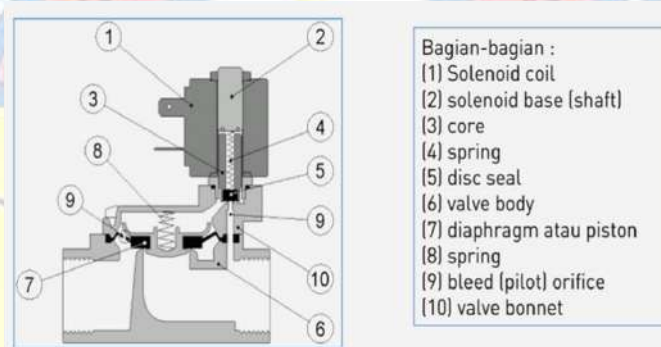
Gambar5. 19 Bagian-bagian Solenoid Valve
