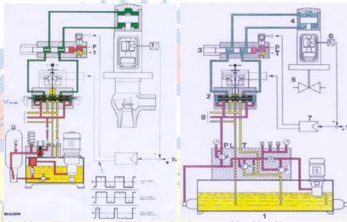
Gambar5. 17 Servo valve
