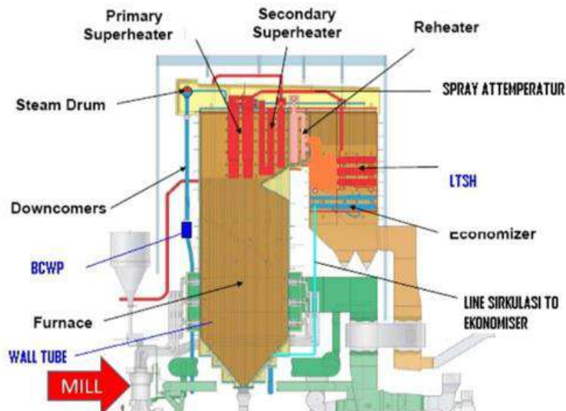
Gambar3.3 BOILER
