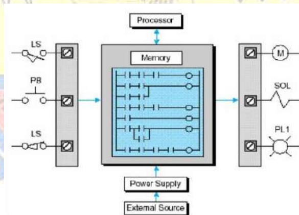
Gambar5. 3Hirarki PLC
