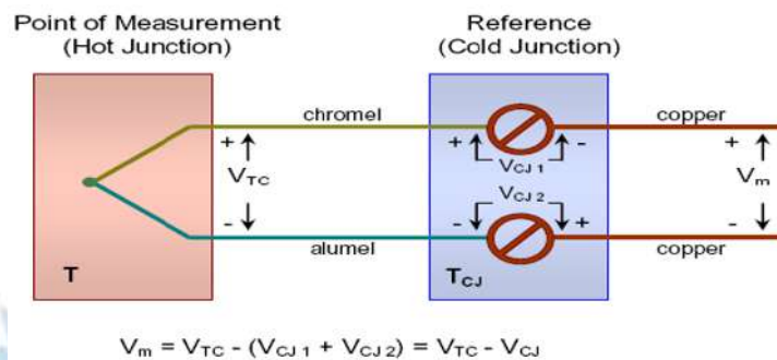
Gambar5. 12 Rangkaian Thermocouple
