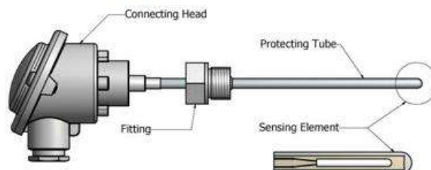
Gambar5. 11 Thermocouple (T/C)
