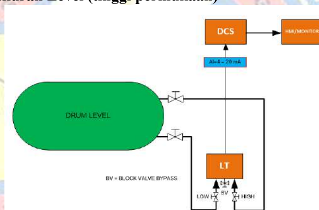
Gambar5. 6 Instalasi level transmitter
