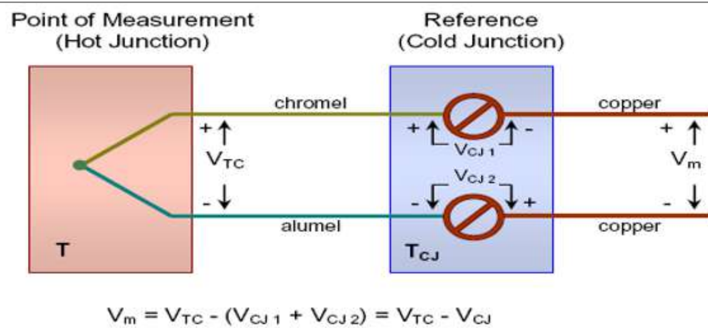
Gambar5. 12 Rangkaian Thermocouple
