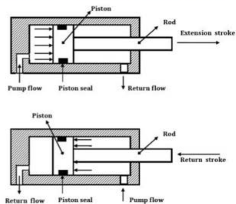
Gambar5. 14 Piston Double Acting
