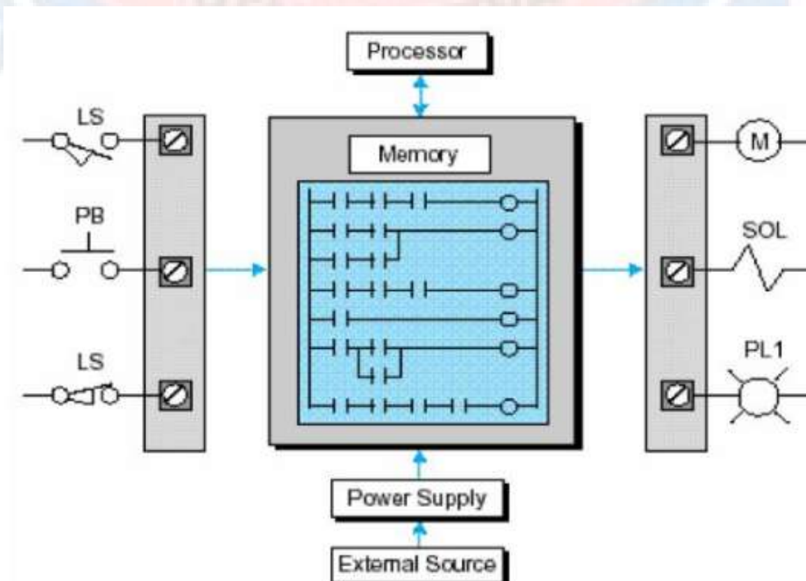
Gambar5. 3Hirarki PLC
