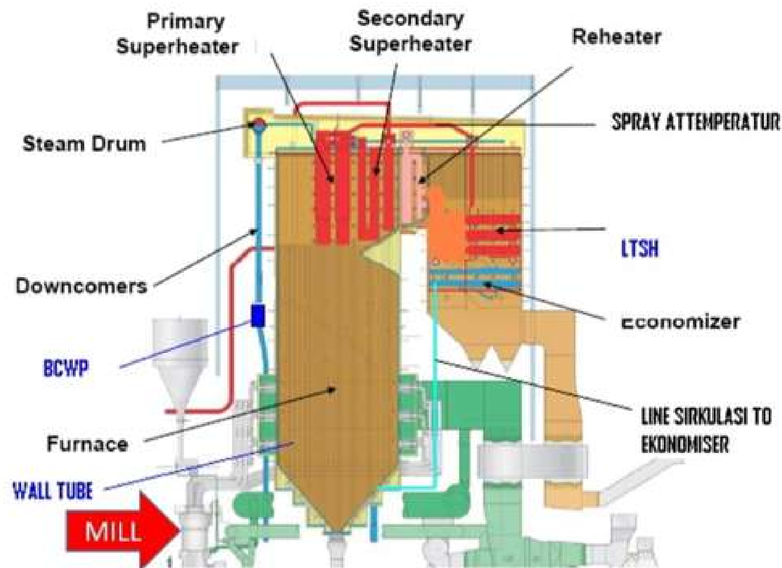
Gambar3.3 BOILER
