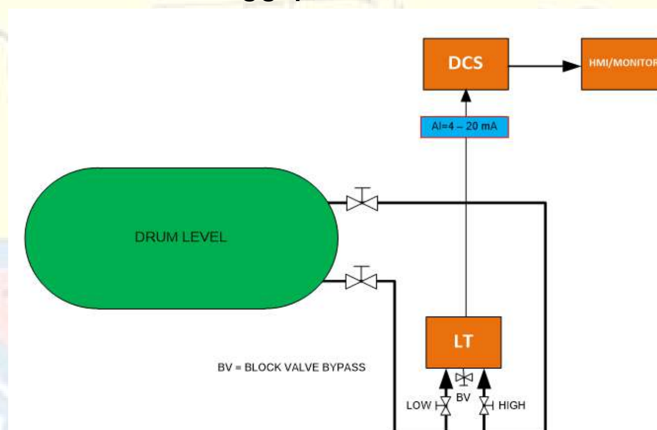
Gambar5. 6 Instalasi level transmitter
