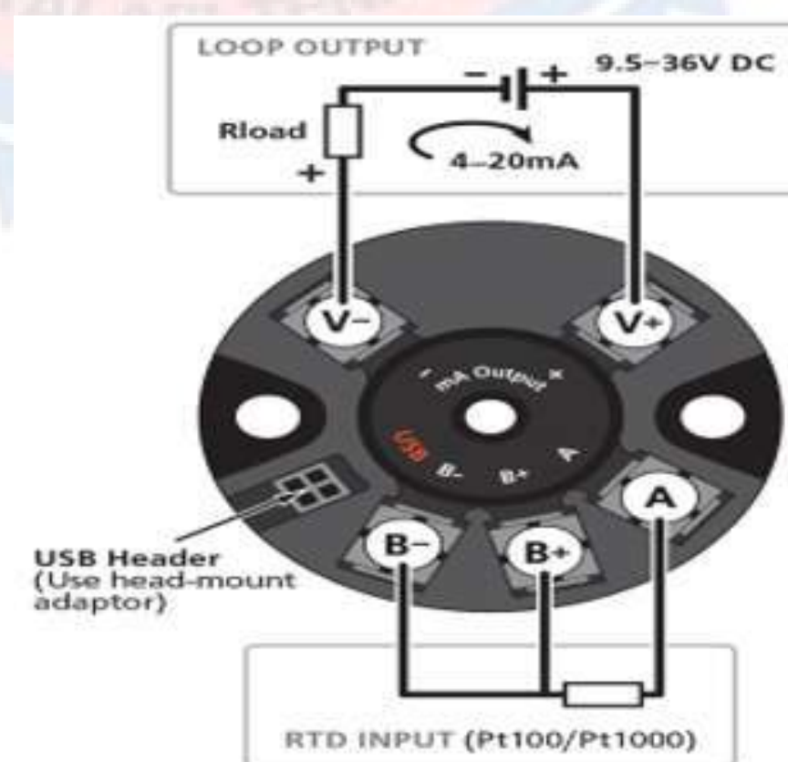
Gambar5. 10 RTD (Resistance Temperature Detector)
