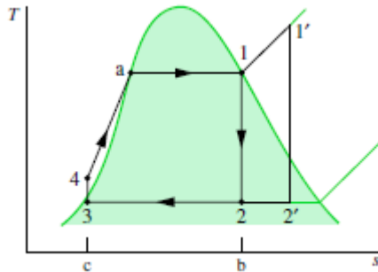
Gambar 3. 3 T-S Diagram
