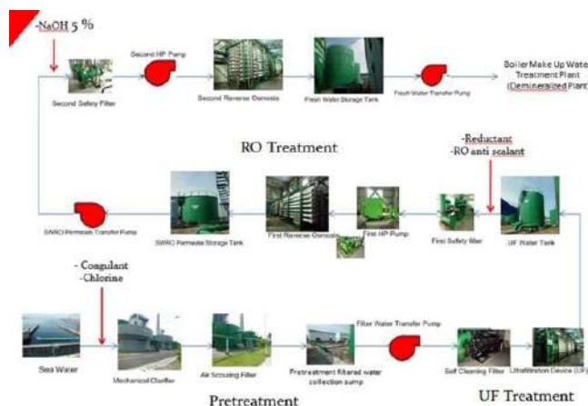
Gambar 3.5 Siklus Water Treatment Plant
