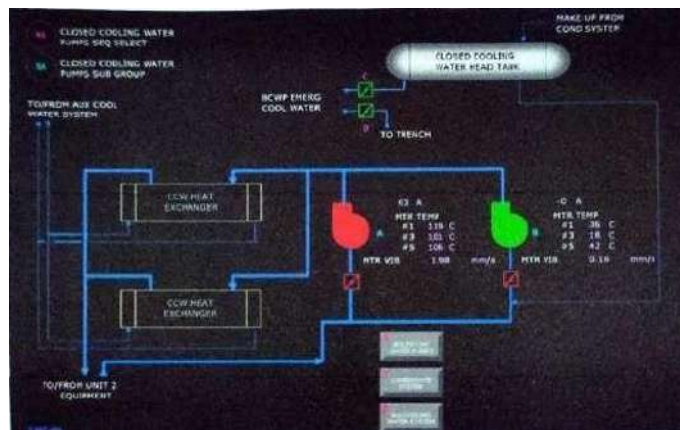
Gambar 3.12 Siklus Closed Cooling
