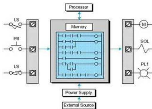
Gambar: 5.3 HIRARKI PLC
