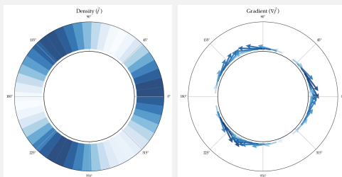
3 Estimated marginal density \hat{f} and gradient \nabla \hat{f}
