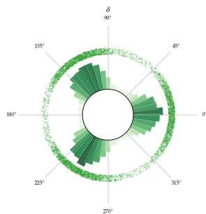
5 Denoised estimates \delta(X)
