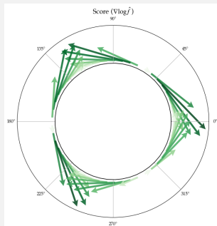
4 Estimated score field \sigma^2 \nabla \log \hat{f}
