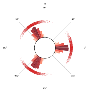
1 Latent truths \Theta \sim G on S^1
