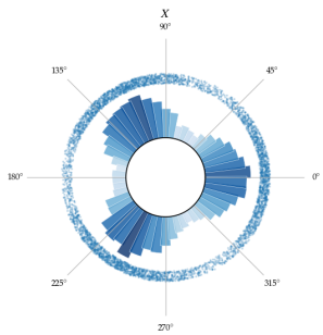
2 Observations X \sim \mathcal{N}(\Theta, \sigma^2)
