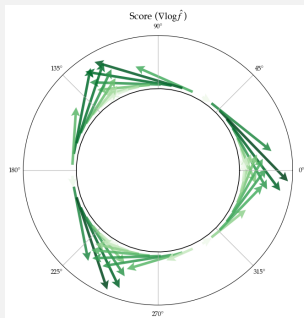
4 Estimated score field \sigma^2 \nabla \log \hat{f}
