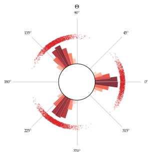
1 Latent variables \Theta \sim G
