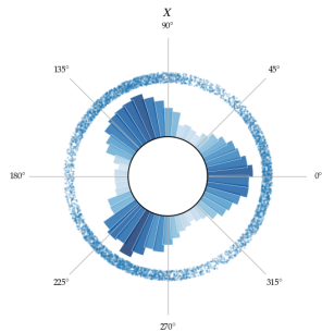
2 Measurements X \sim \mathcal{N}(\Theta, \sigma^2)
