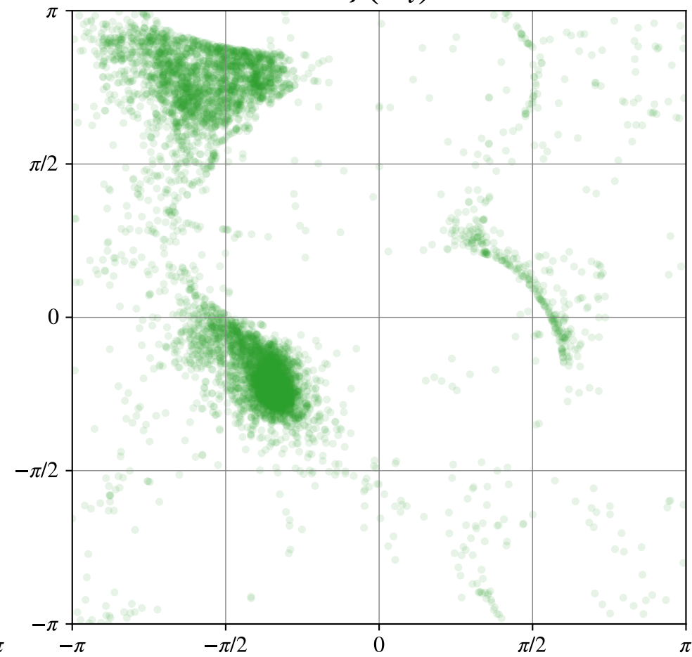
\hat{\delta}_{\mathcal{T}}(X_i)
