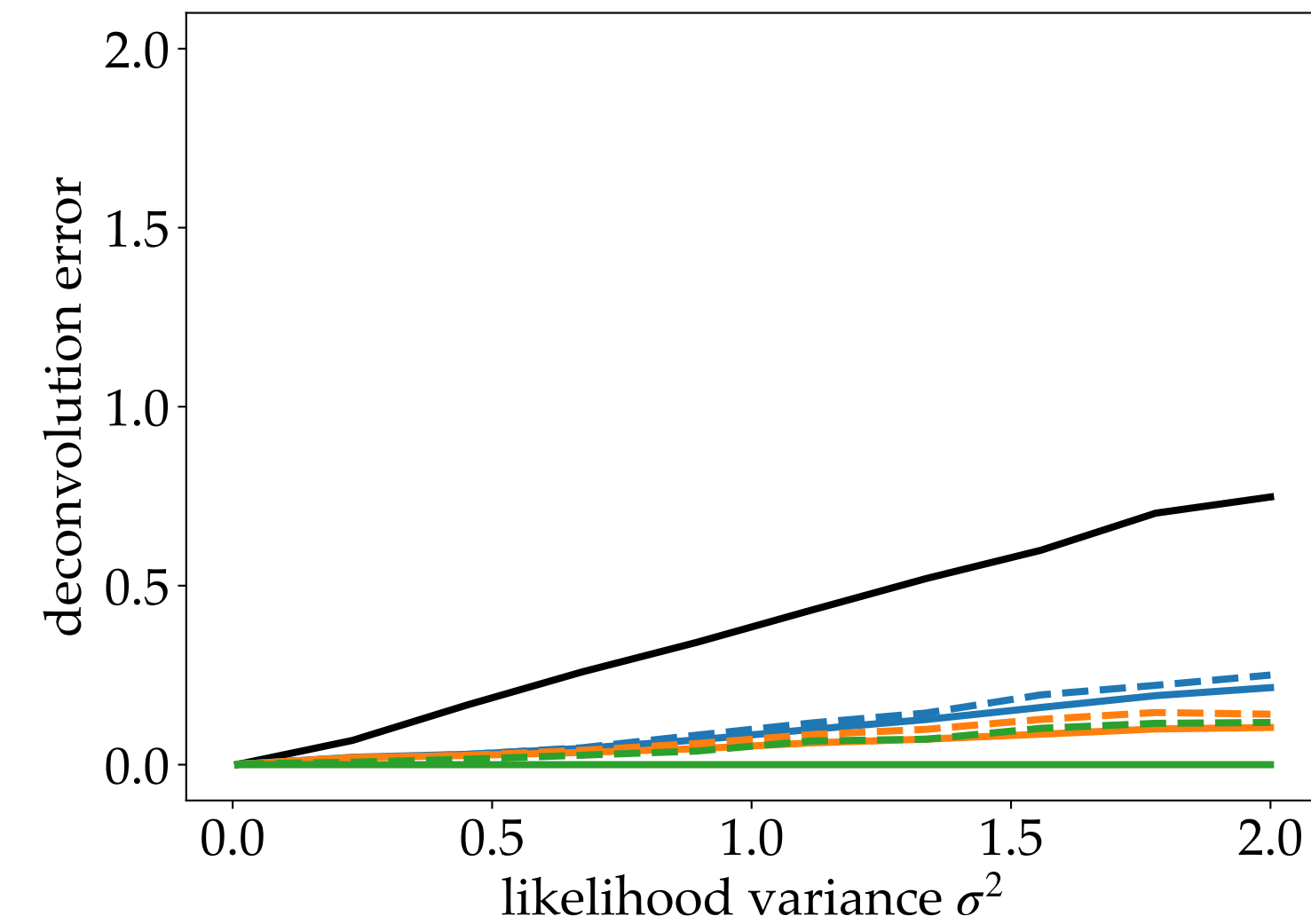
varying \sigma^2 with fixed \tau^2 = 0.2
