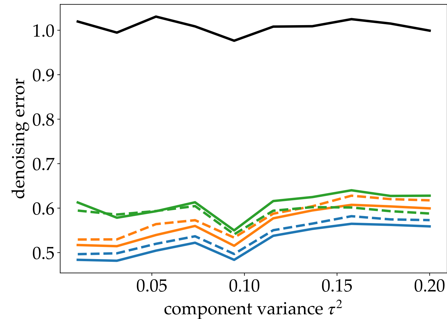
varying \tau^2 with fixed \sigma^2 = 1.0
