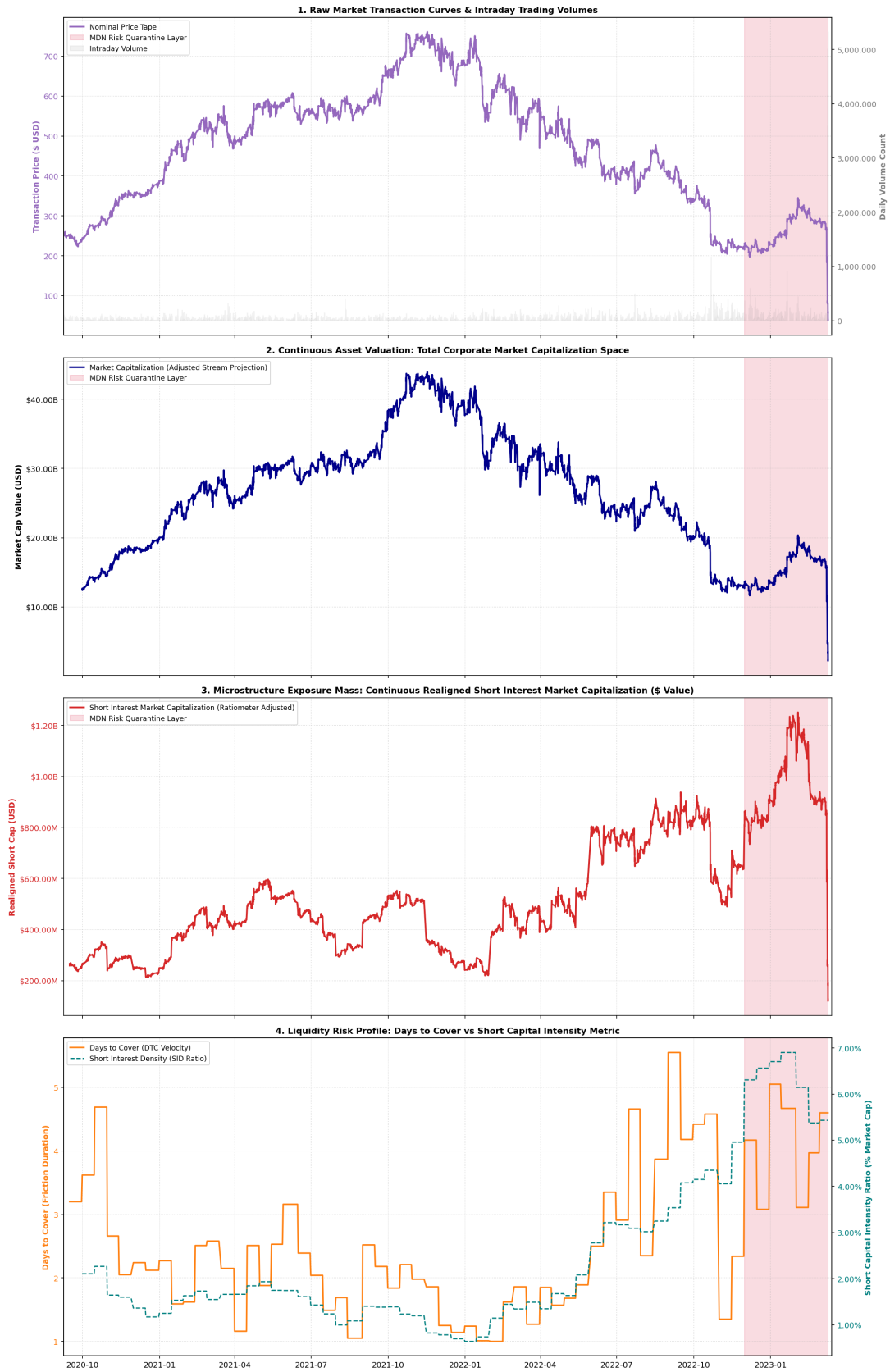
Figure 9: Arithmetic telemetry profile for Silicon Valley Bank (SIVB).
