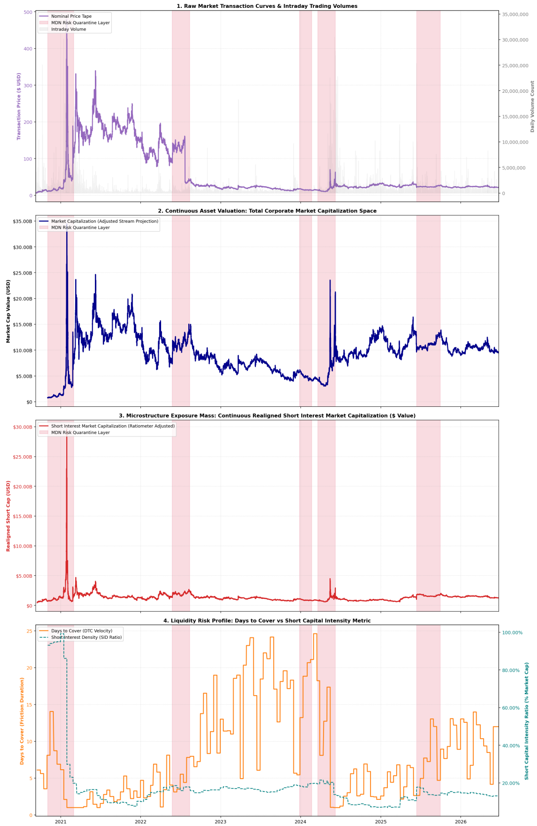
Figure 7: Arithmetic telemetry profile for GameStop (GME).
