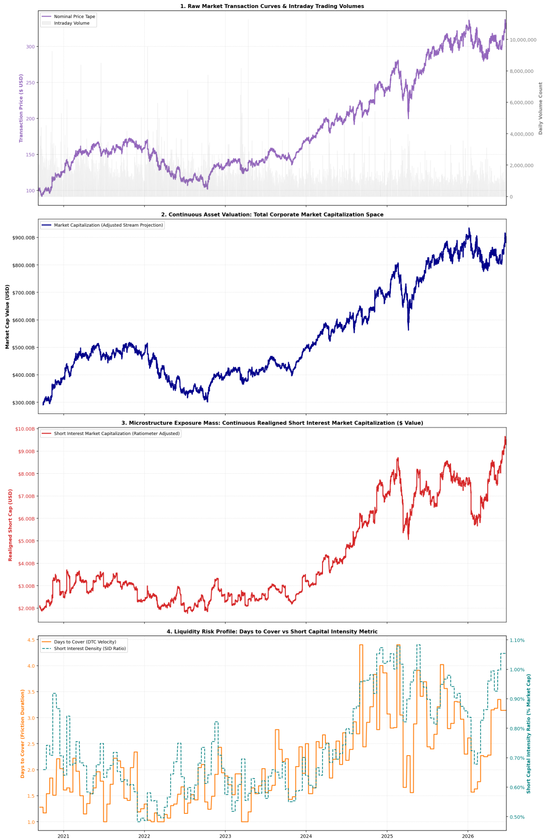
Figure 8: Arithmetic telemetry profile for JPMorgan Chase (JPM).
