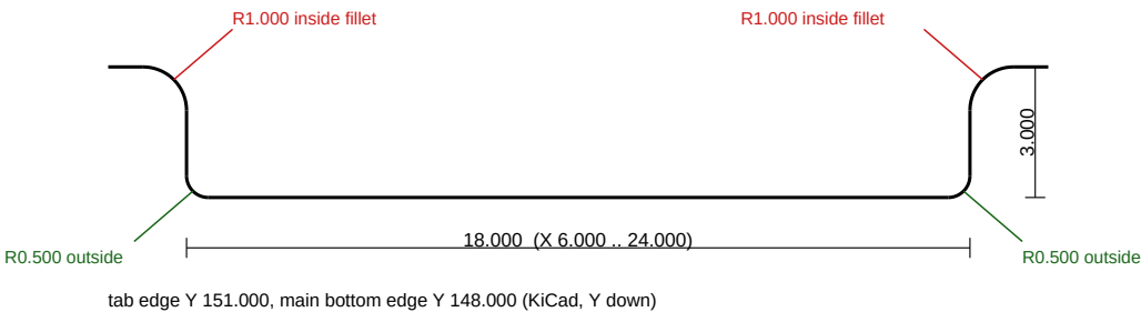
DETAIL J2_TAB (scale 5.2 : 1)
