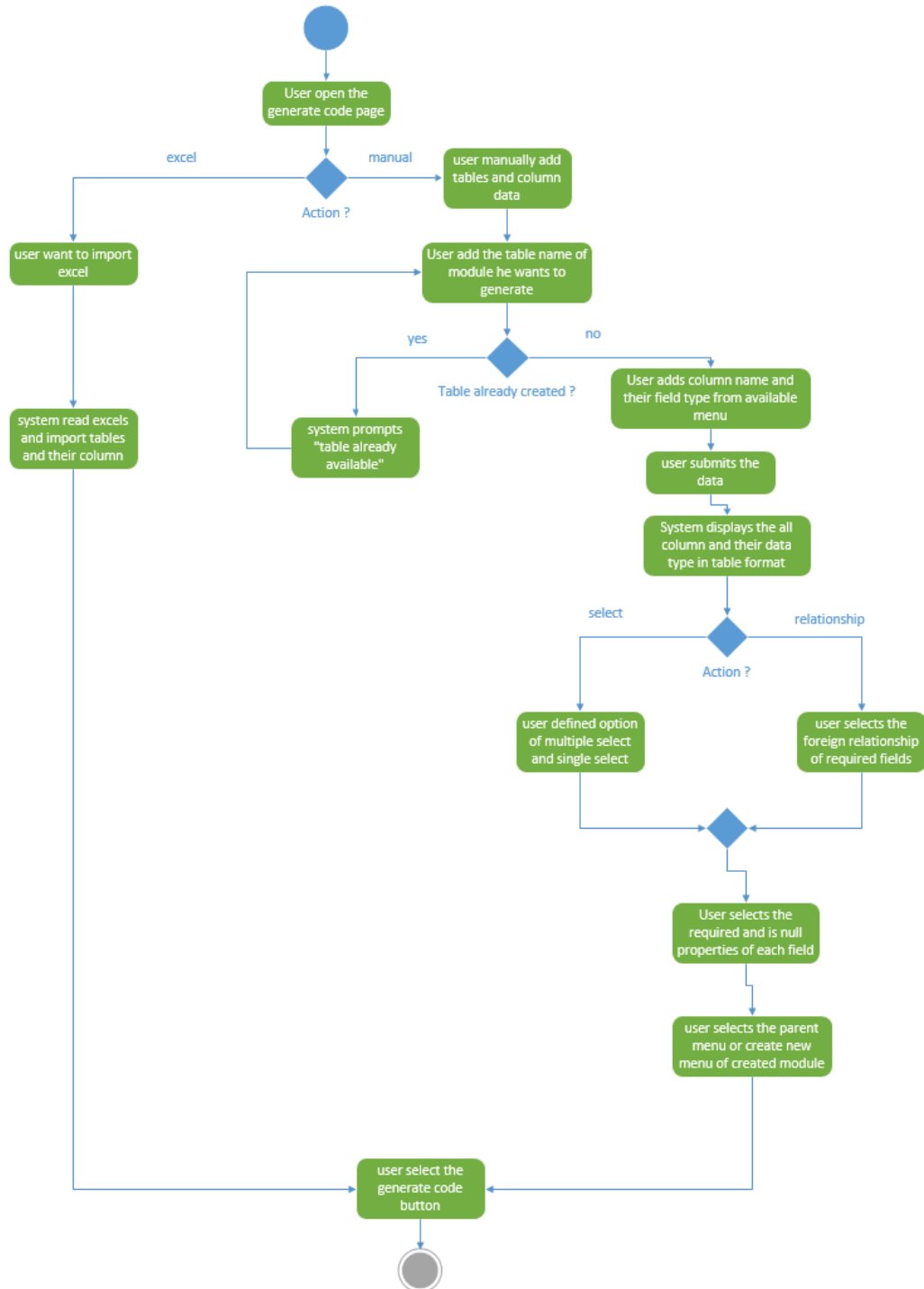
Figure 4-6 Integration and development Activity Diagram
