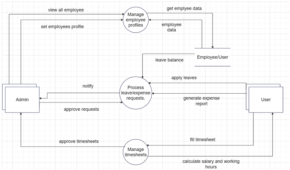
Figure 4-22 HR management Level 2 DFD
