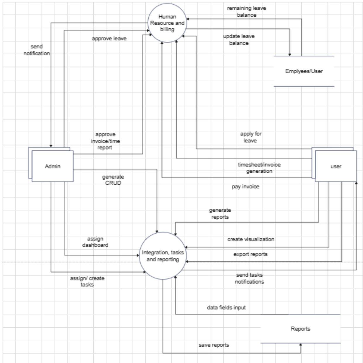
Figure 4-19 Development and HR management Level 1 DFD
