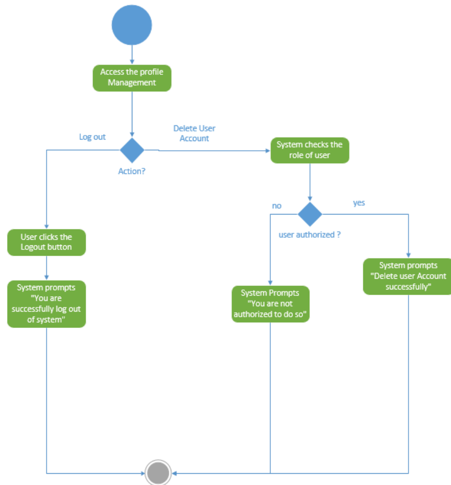
Figure 4-4 Delete User Account Activity Diagram
