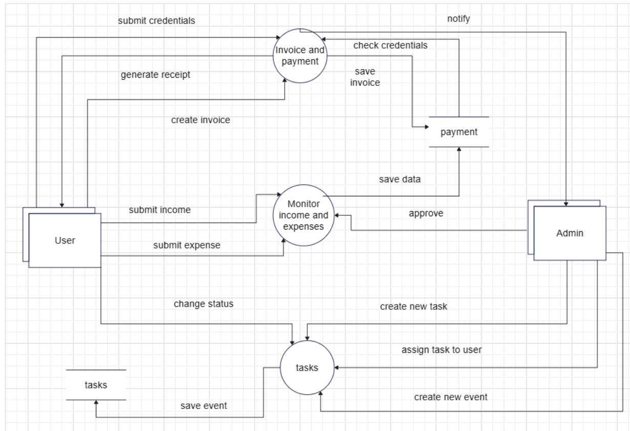
Figure 4-24 Task and billing Management Level 2 DFD
