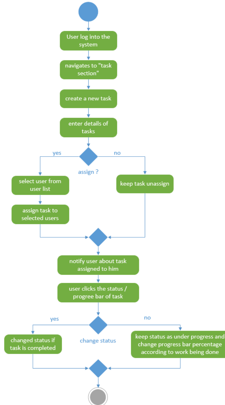
Figure 4-15 Task management Activity Diagram
