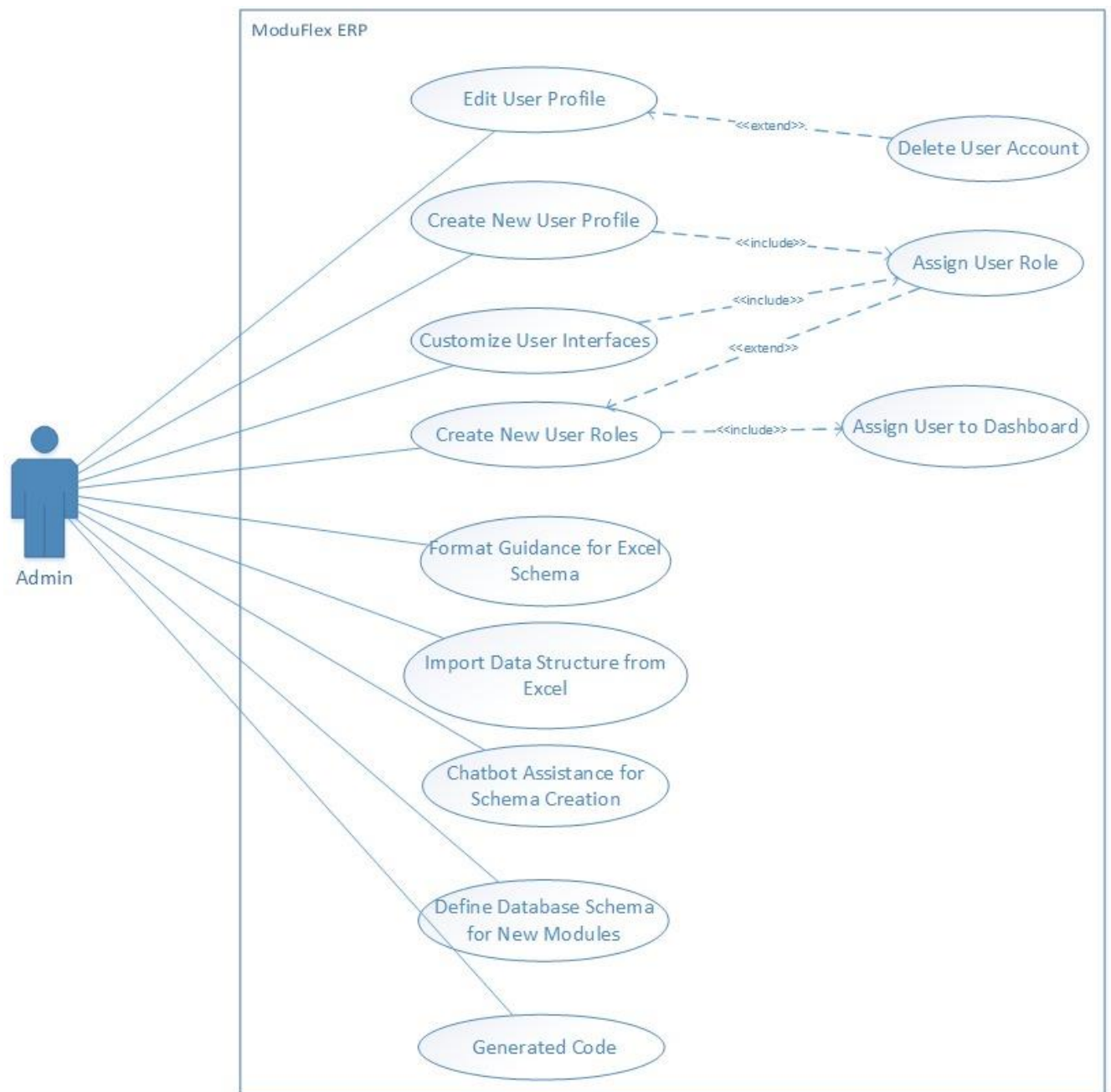
Figure 3-2 Use case Diagram for Admin
