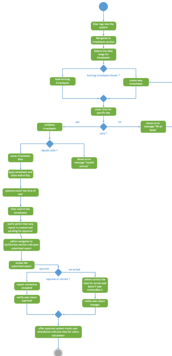
Figure 4-10 Timesheets Activity Diagram
