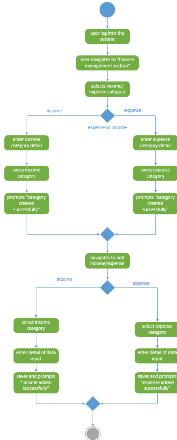
Figure 4-14 Financial Inputs Activity Diagram
