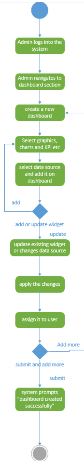
Figure 4-12 Dashboard creation Activity Diagram
