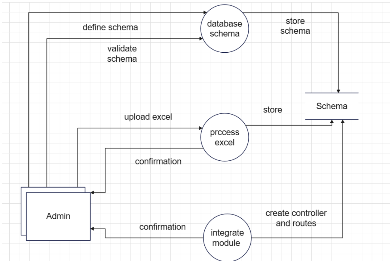
Figure 4-21 Integration and Development Level 2 DFD
