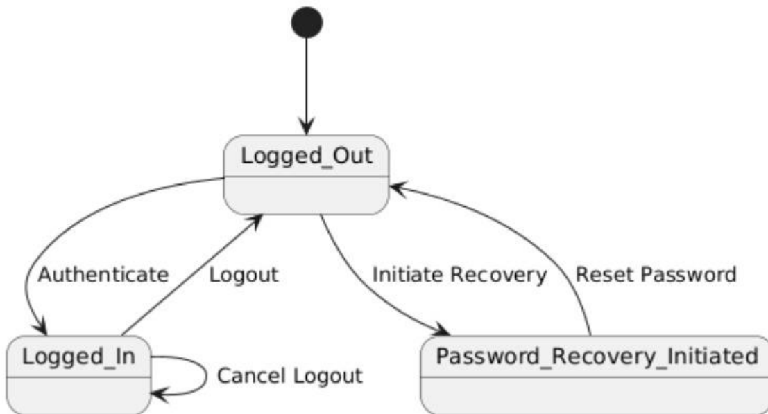
Figure 4-25 STATE TRANSITION DIAGRAM user authentication
