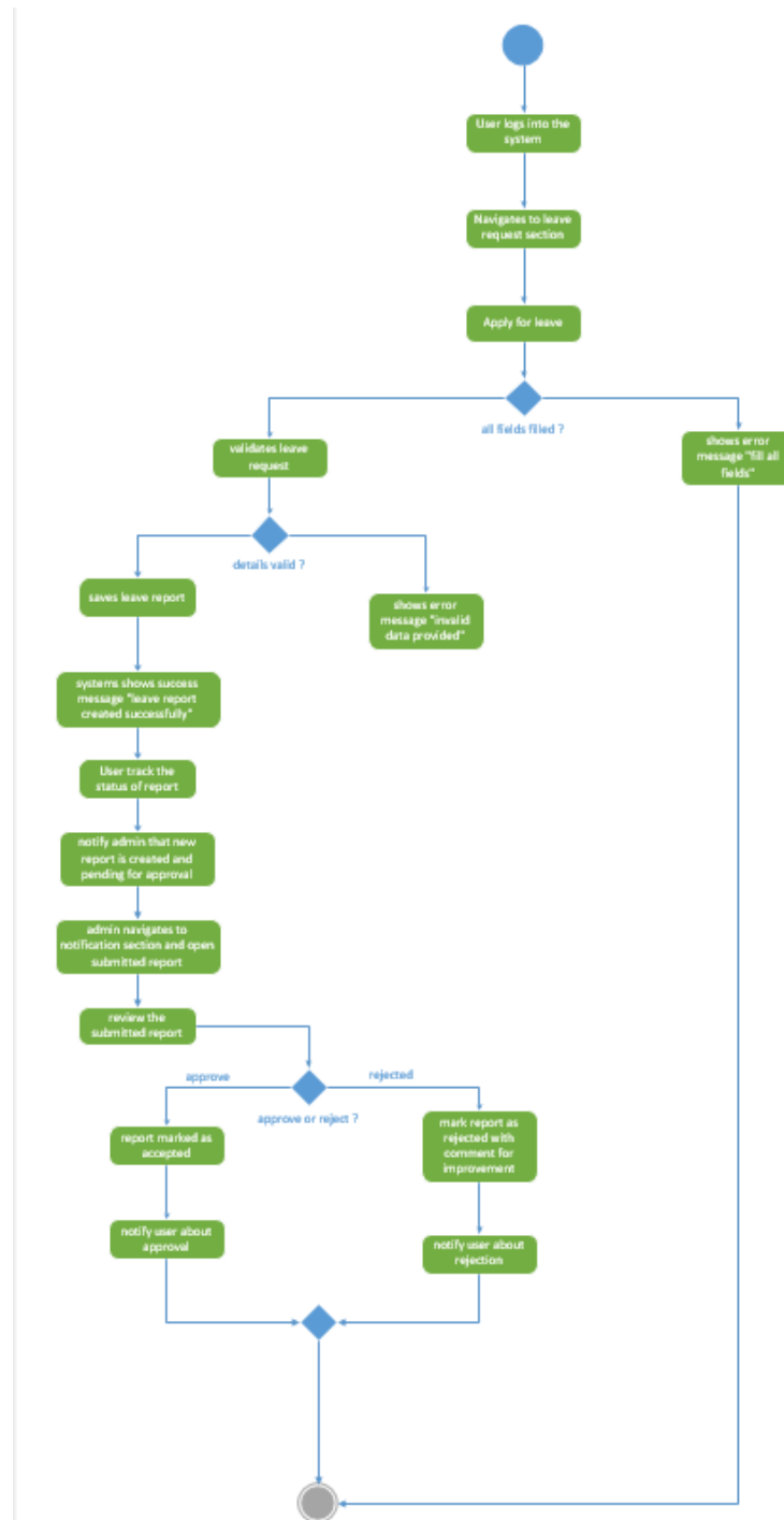
Figure 4-9 Leave Request Activity Diagram
