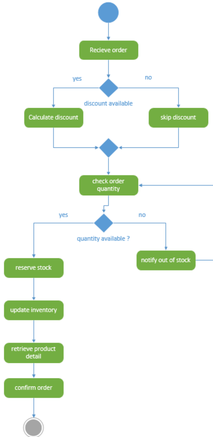
Figure 4-16 Order Management Activity Diagram
