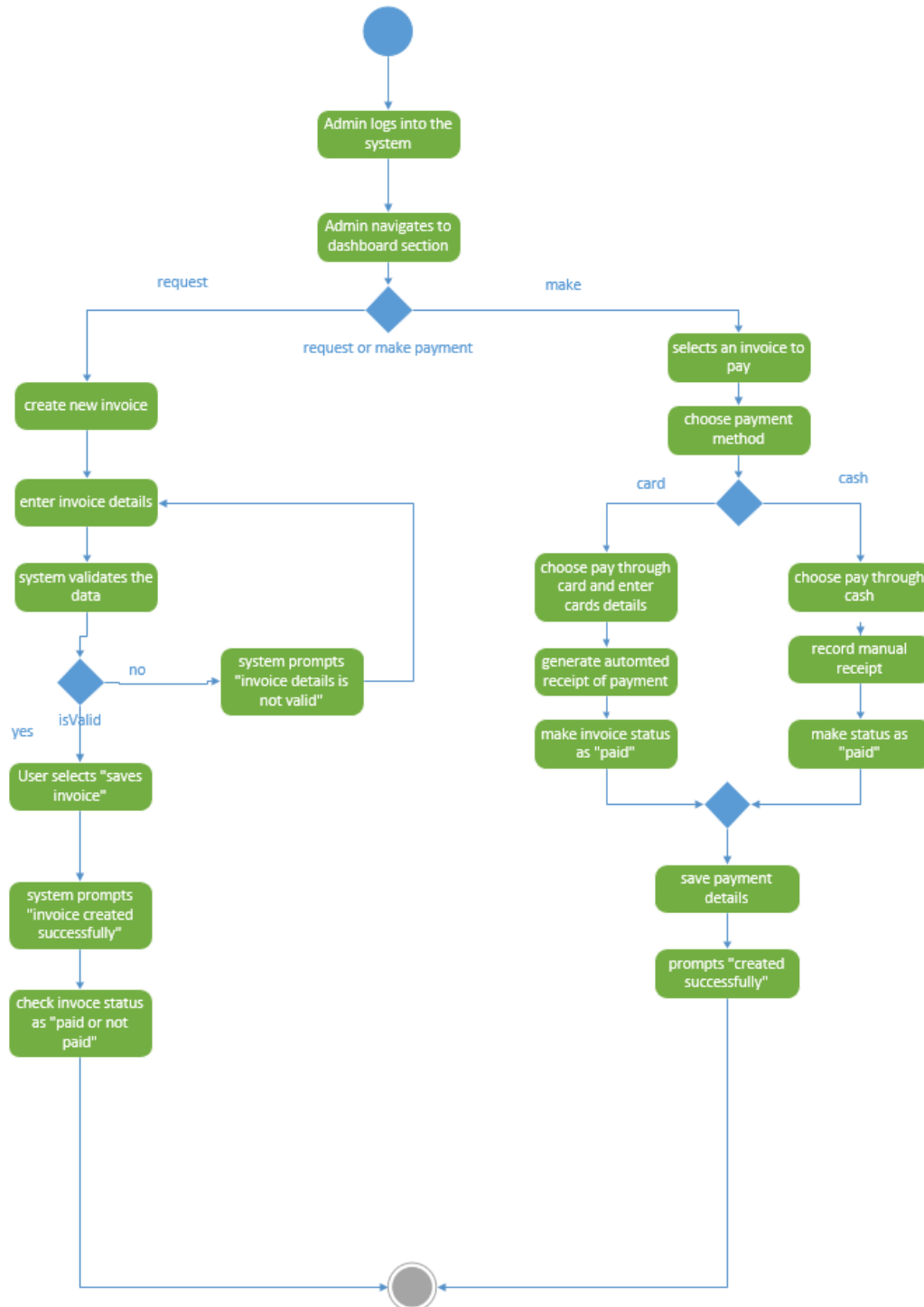
Figure 4-13 Invoices and payment Activity Diagram
