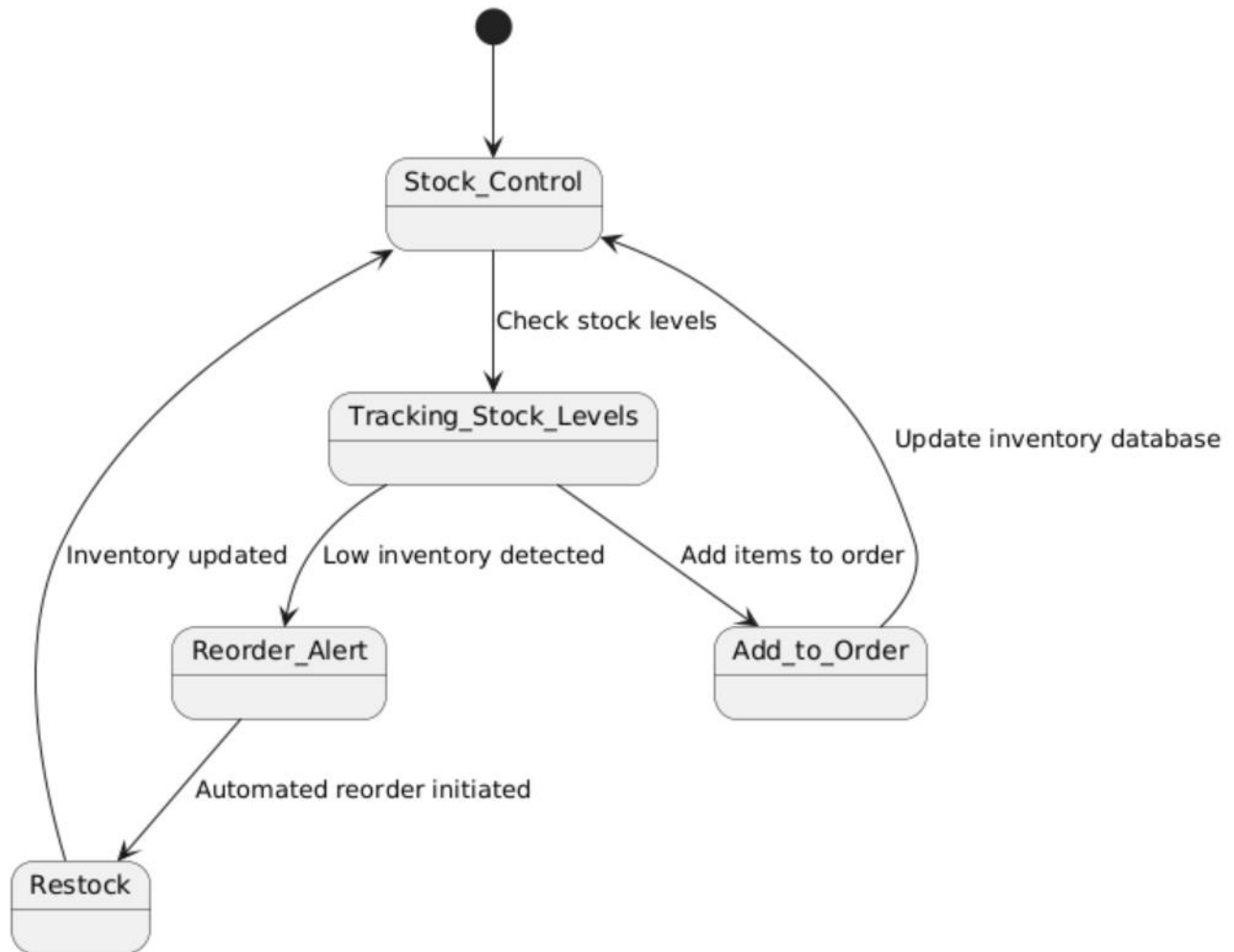
Figure 4-32 STATE TRANSITION DIAGRAM Inventory management
