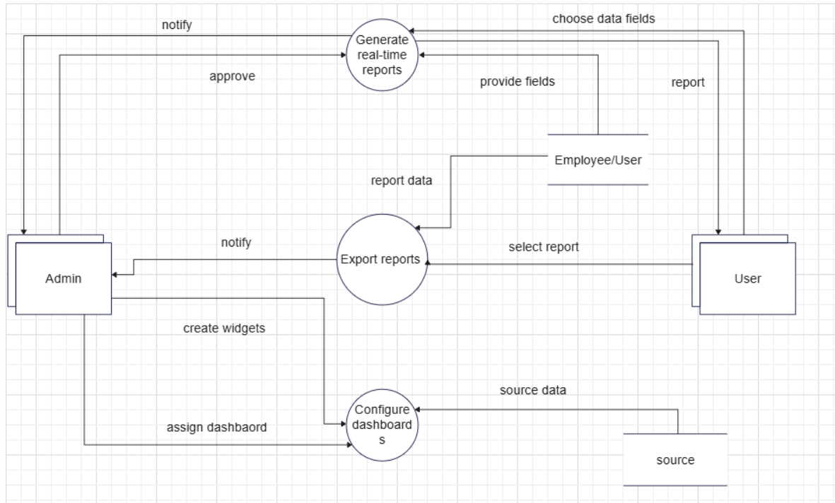
Figure 4-23 Dashboard Level 2 DFD
