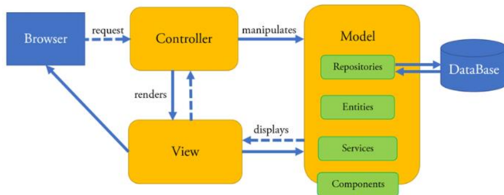
Figure 4-1 MVC Diagram of ModuFlex ERP System
