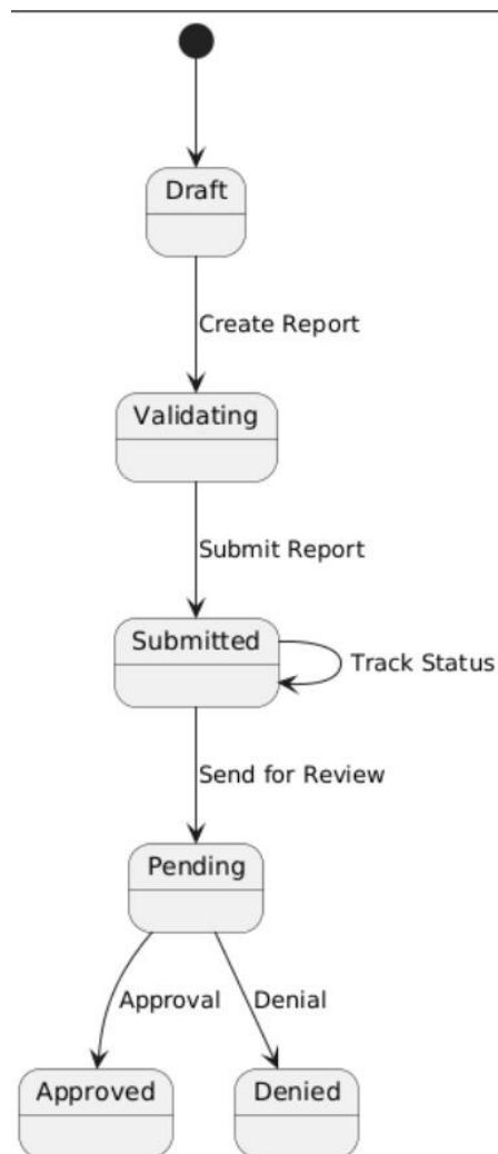
Figure 4-27 STATE TRANSITION DIAGRAM submit and track expense report
