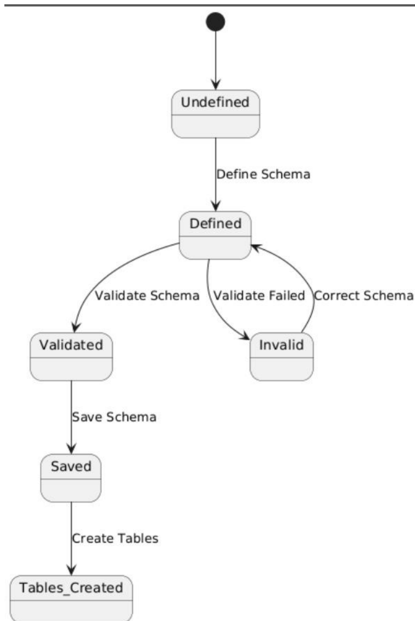
Figure 4-26 STATE TRANSITION DIAGRAM database schema generation
