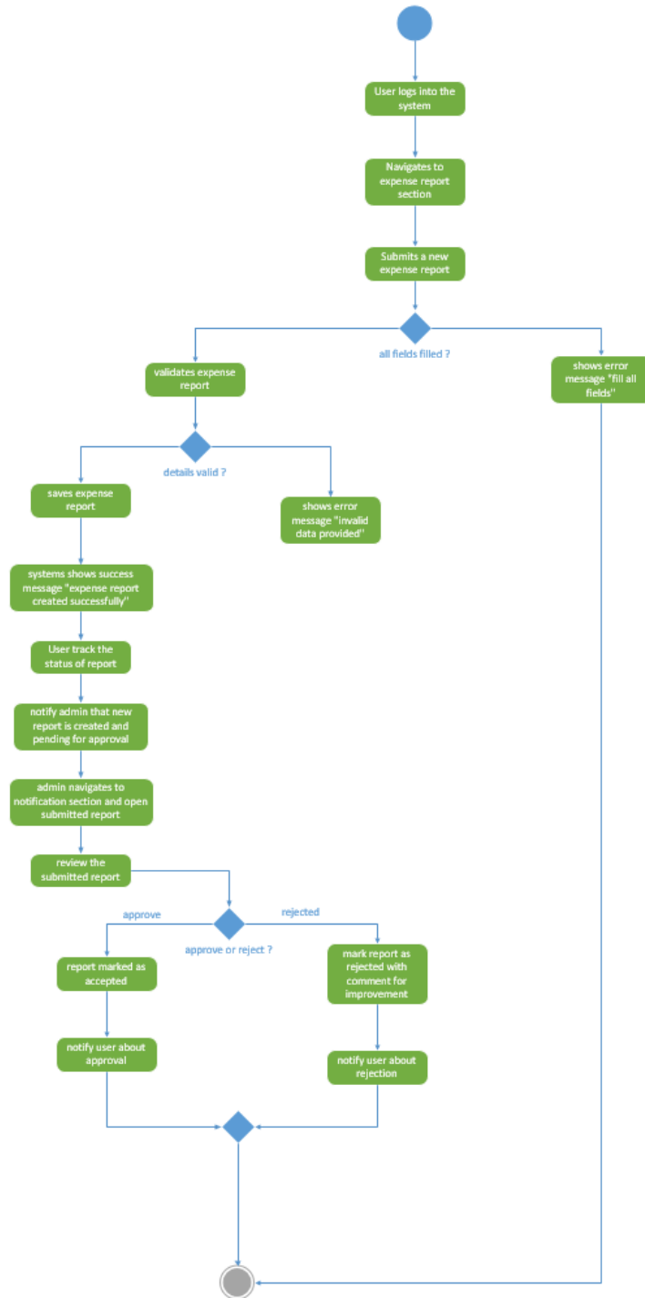
Figure 4-8 Submit and track expense report Activity Diagram
